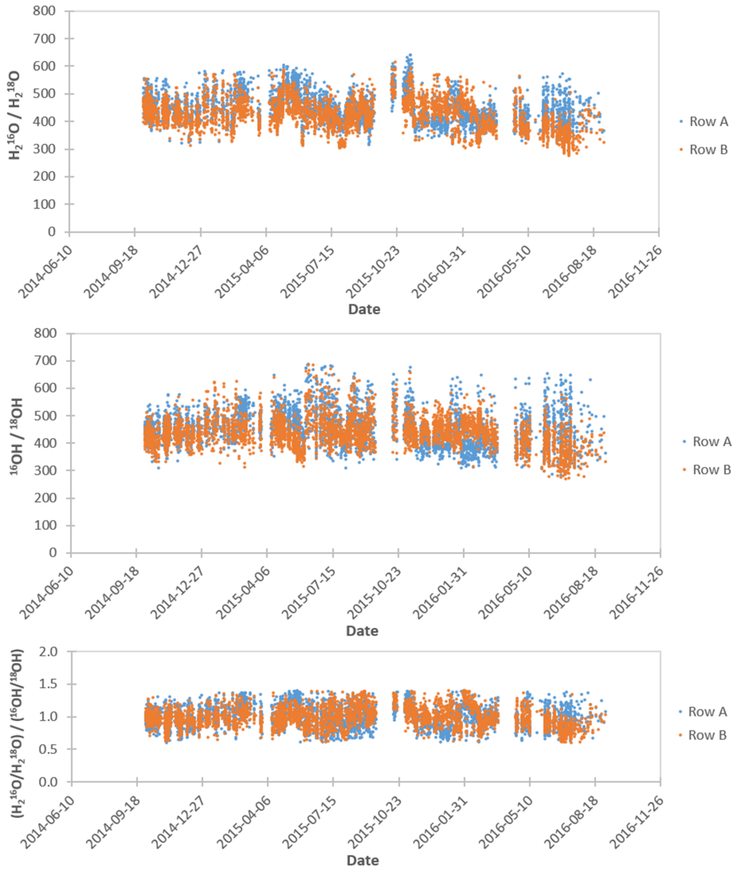
Fig. 1. \text{H}_2^{16}\text{O}/\text{H}_2^{18}\text{O} ratio (top), ^{16}\text{OH}/^{18}\text{OH} ratio (middle), and \frac{\text{H}_2^{16}\text{O}/\text{H}_2^{18}\text{O}}{^{16}\text{OH}/^{18}\text{OH}} ratio (bottom) over the course of the mission. See Fig. A.4 for an idea of the typical error bars on a single isotopic ratio measurement.
