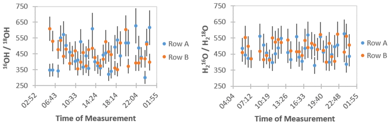
Fig. A.4. ^{16}\text{OH}/^{18}\text{OH} (left) and \text{H}_2^{16}\text{O}/\text{H}_2^{18}\text{O} (right) measured during the sniff test on 19 June 2014. Error bars reflect the uncertainties in the gain (6%) and pixel gain (5%) and the counting error.
