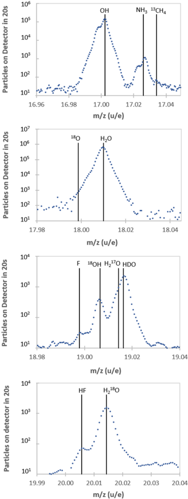
Fig. A.2. Sample DFMS mass spectra (from 2014-10-20) for m/z 17–20 u/e.
