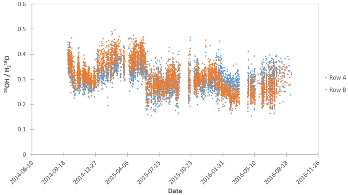
Fig. A.3. Uncorrected ^{18}\text{OH}/\text{H}_2^{18}\text{O} plotted against time of measurement.
