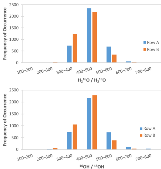
Fig. 2. Histograms of individual measurements. Top: H_2^{16}O/H_2^{18}O . Bottom: ^{16}OH/^{18}OH .
