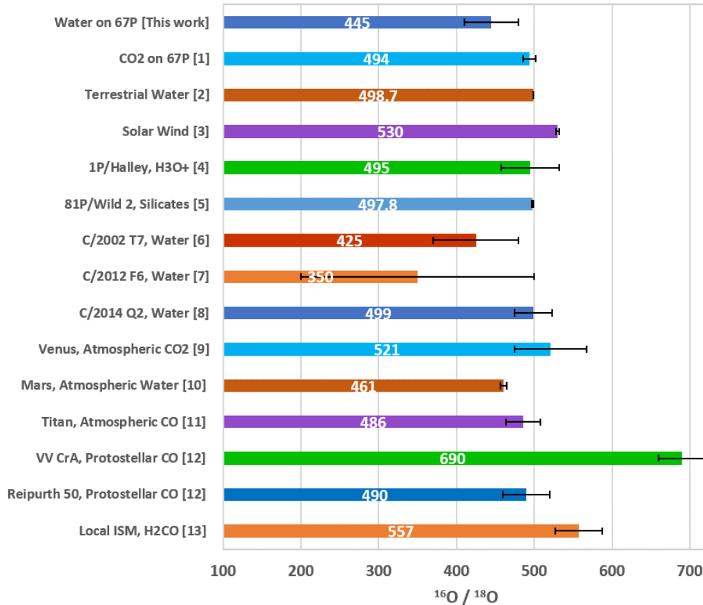
Fig. 3. Comparison of ^{16}\text{O}/^{18}\text{O} ratios from various sources. References: (1) Hässig et al. (2017); (2) Baertschi (1976); (3) McKeegan et al. (2011); (4) Eberhardt et al. (1995); Balsiger et al. (1995); (5) Ogliore et al. (2015); (6) Hutsemékers et al. (2008); (7) Decock et al. (2014); (8) Biver et al. (2016); (9) Iwagami et al. (2015); (10) Webster et al. (2013); (11) Serigano et al. (2016); (12) Smith et al. (2009); (13) Wilson (1999).
