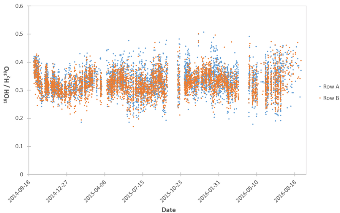
Fig. A.5. Corrected ^{18}\text{OH}/\text{H}_2^{18}\text{O} plotted against time of measurement.
