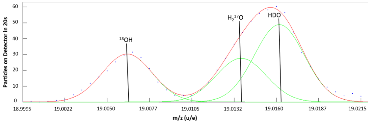
Fig. 4. Sample DFMS mass spectrum from 2016-03-03 T 03:45 illustrating the use of manual peak-fitting with equal-width Gaussians to separate the \text{H}_2^{17}\text{O} peak from that of HDO. Dotted line: mass spectrum, green lines: fitted Gaussians, red line: sum of fitted Gaussians.
