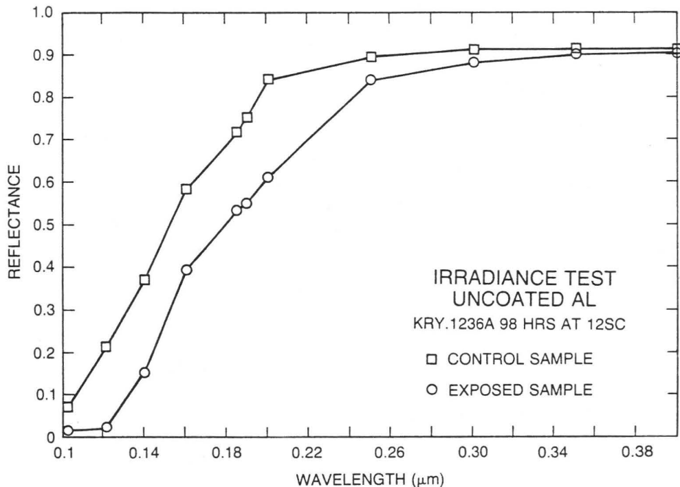
Figure 2.2 Reflectivity as a function of wavelength for uncoated aluminum surfaces, one of which was exposed to an oil-pumped vacuum system, and the other (control sample) not.
