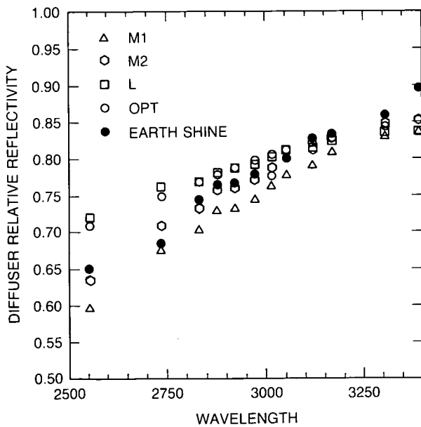
Figure 2.18b As in 18a, but for December 1984.
