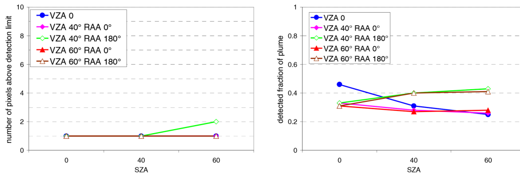
(c) number of pixels above the detection limit for BrO (340 nm) (d) retrieved fraction of the plume content for BrO (340 nm)
