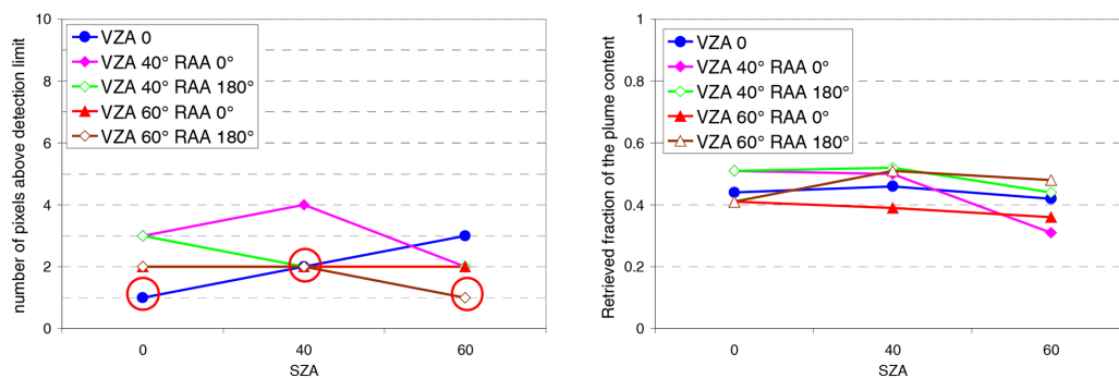
(e) number of pixels above the detection limit for IO (440 nm) (f) retrieved fraction of the plume content for IO (440 nm)
