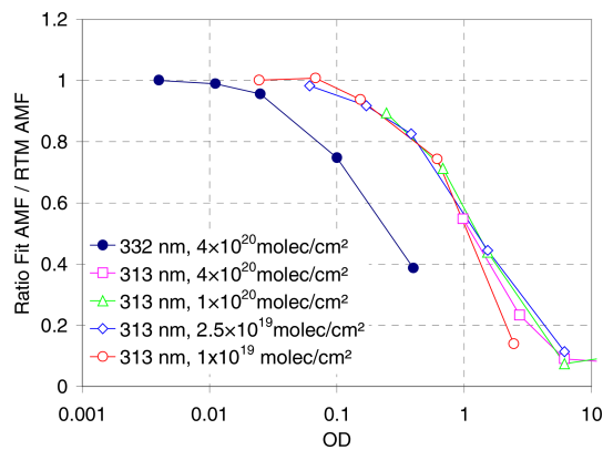
Figure D2. Ratio between true AMFs and monochromatic AMFs as a function of the vertical optical depth of SO 2 in the plume.
