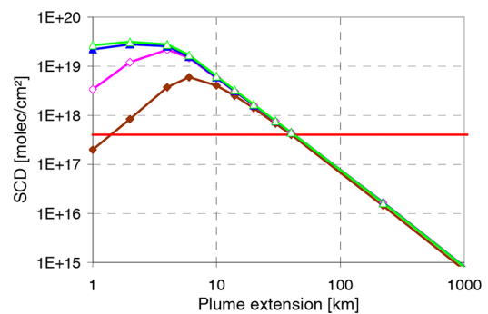
Figure C5. Same as Fig. 14 but for additional plume heights: retrieved fraction of the plume content (top) and \text{SO}_2 SCDs (bottom) from TROPOMI measurements at different wavelengths as a function of the plume size and for different amounts of molecules in the plume. The red horizontal line indicates the threshold, above which the operational \text{SO}_2 retrieval switches from the standard fit window to the first alternative fit window (at longer wavelengths).
