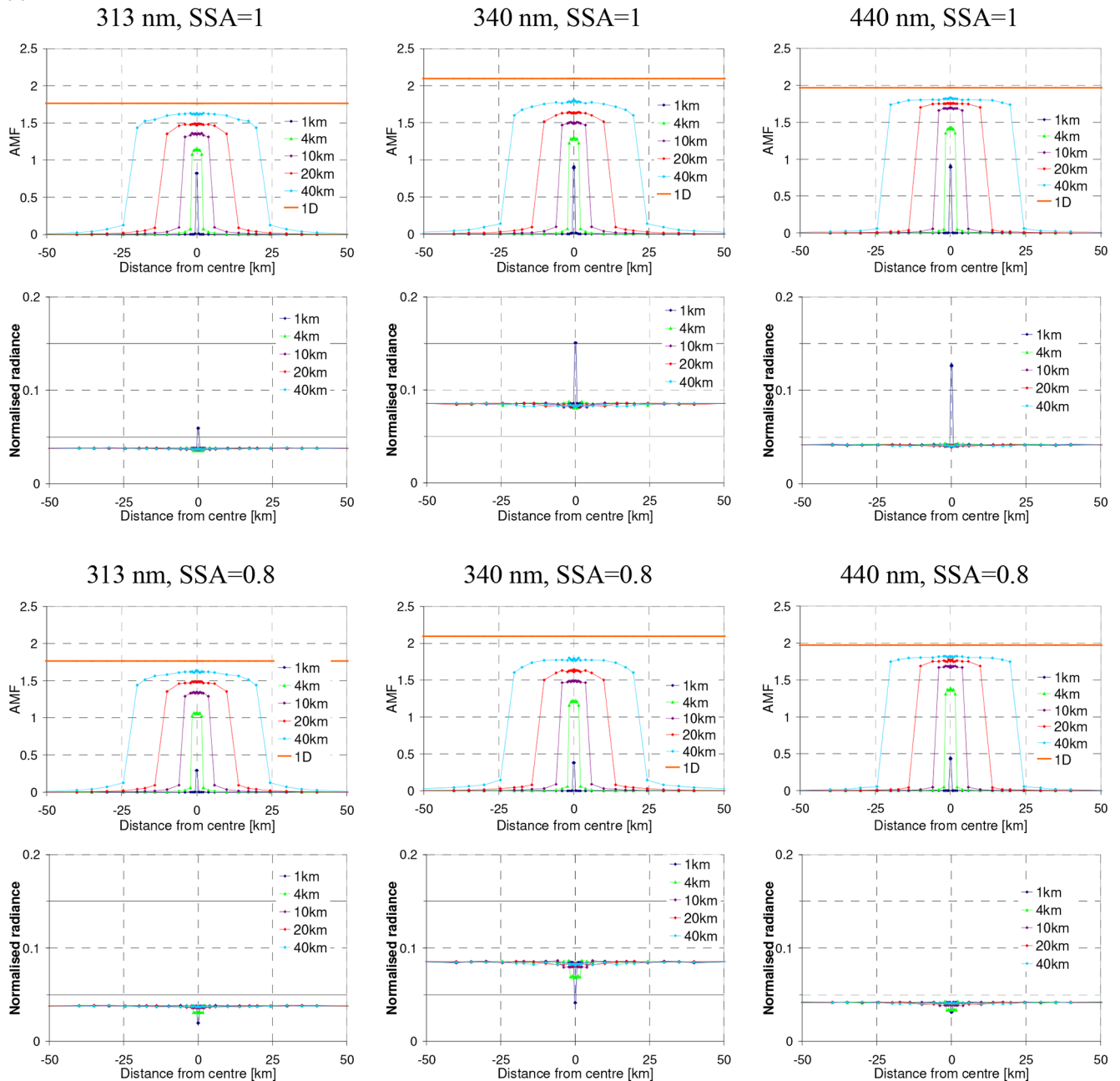
Figure C3. Same as Fig. 11 but for additional plume heights: AMFs and normalised radiances for plume scans in near-nadir viewing geometry ( SZA = 0^\circ ) for different wavelengths and aerosol contents. The satellite scans the plume with a narrow FOV ( \sim 0.014^\circ ). The different colours represent AMFs for plumes with different horizontal extensions (from 1 \times 1 to 40 \times 40 \text{ km}^2 ). The rather low radiance at 313 nm (in spite of the high probability of Rayleigh scattering) is caused by the stratospheric ozone absorption.
