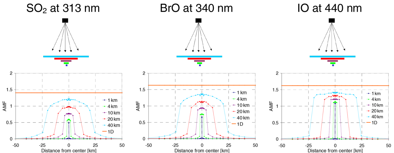
Figure 6. AMFs for plume scans in near-nadir viewing geometry (SZA = 0°, VZA = 0°) at different wavelengths. It is assumed that the satellite scans the plume with a narrow FOV ( \sim 0.014^\circ ). The different colours represent AMFs for plumes at 5–6 km altitude and with different horizontal extensions (from 1 \times 1 \text{ km}^2 to 40 \times 40 \text{ km}^2 ). Results for other plume altitudes are shown in Appendix C.
