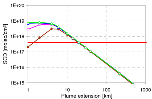
Figure C5. Same as Fig. 14 but for additional plume heights: retrieved fraction of the plume content (top) and \text{SO}_2 SCDs (bottom) from TROPOMI measurements at different wavelengths as a function of the plume size and for different amounts of molecules in the plume. The red horizontal line indicates the threshold, above which the operational \text{SO}_2 retrieval switches from the standard fit window to the first alternative fit window (at longer wavelengths).
