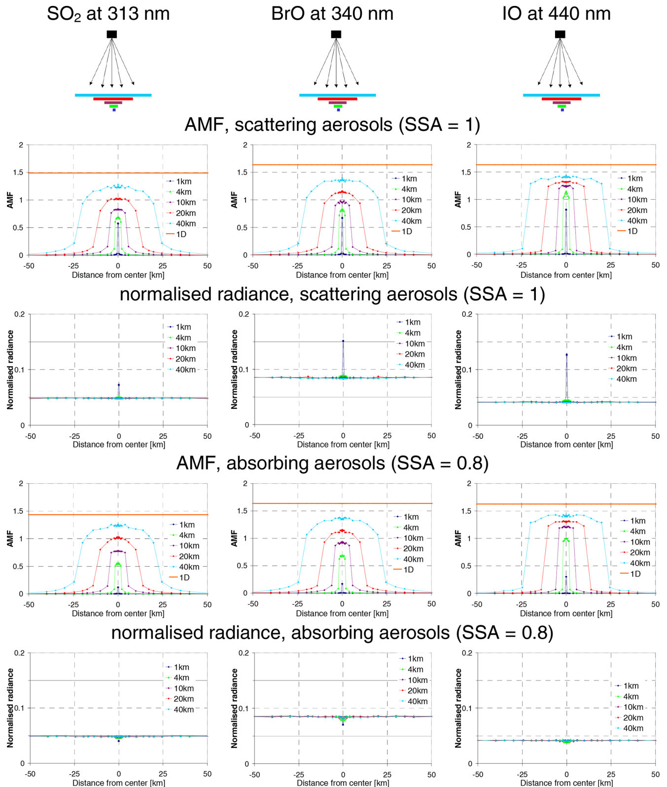
Figure 11. AMFs and normalised radiances for plume scans in near-nadir viewing geometry ( \text{SZA} = 0^\circ ) for different wavelengths and aerosol contents. The satellite scans the plume with a narrow FOV ( \sim 0.014^\circ ). The different colours represent AMFs for plumes at 5–6 km altitude and with different horizontal extensions (from 1 \times 1 to 40 \times 40 \text{ km}^2 ). The rather low radiance at 313 nm (in spite of the high probability of Rayleigh scattering) is caused by the stratospheric ozone absorption. Results for other plume altitudes are shown in Appendix C.
