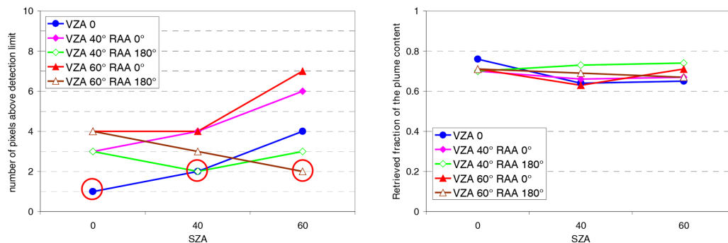
Figure 17. Number of satellite pixels with SCDs above the detection limit (a, c, e) and the retrieved fraction of the plume content (b, d, f) for TROPOMI observations of SO 2 (weak, 313 nm), BrO (340 nm), and IO (440 nm) with different viewing and solar zenith angles. The plume has an extension of 1 \times 1 \times 1 \text{ km}^3 and is located at 5–6 km altitude. The red circles indicate scenarios with the Sun and the satellite in the same direction for which the smearing effect is smallest. RAA indicates the relative azimuth angle between the viewing direction and the Sun. Here a RAA of 180° represents cases where the Sun shines in the same direction as the satellite view.
