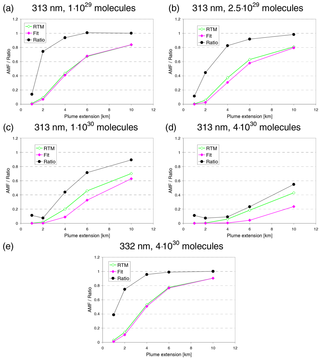
Figure D1. True AMFs (magenta lines) and monochromatic AMFs (green lines) as a function of the horizontal plume extension for different SO 2 scenarios. Also, the ratios of both AMFs are shown (black lines). The AMFs and AMF ratios depend on the wavelength and the SO 2 amount.
