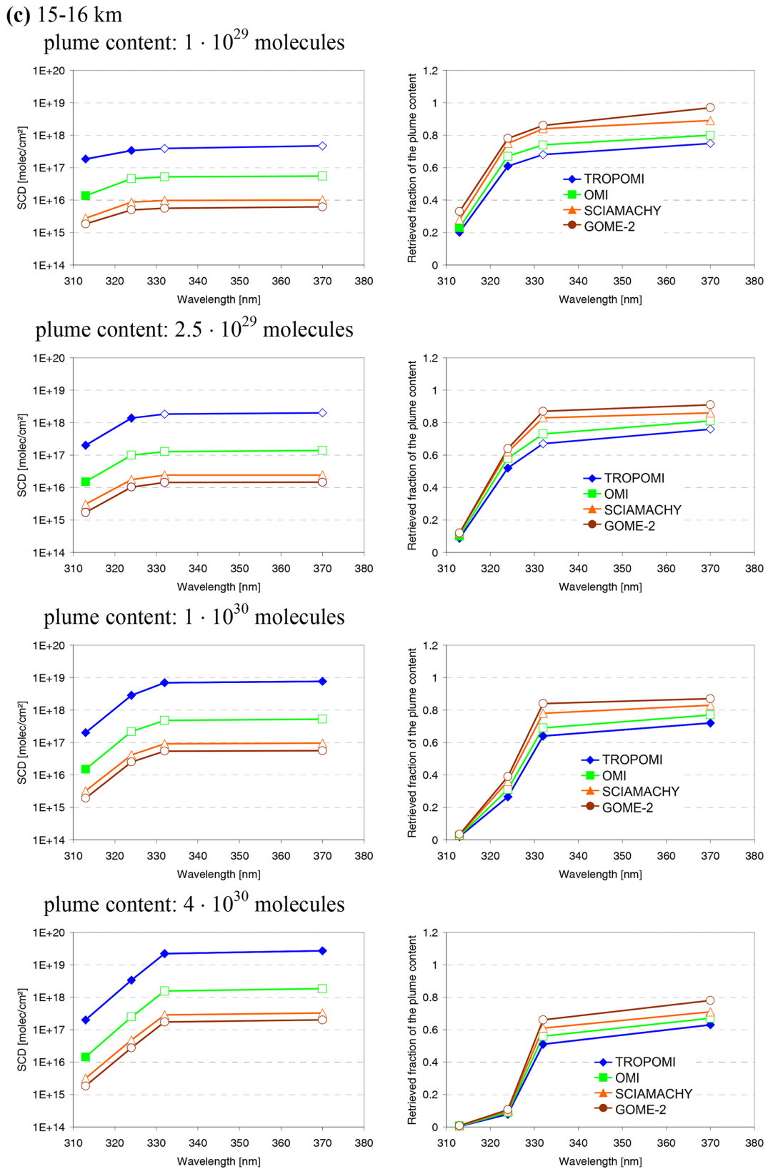
Figure C6. Same as Fig. 15 but for additional plume heights: retrieved fractions of the plume content and SO 2 SCDs for different satellite instruments and for a plume size of 1 \times 1 \text{ km}^2 as a function of the wavelength. The full symbols represent measurements with SCDs above the detection limit. Note that for the rather large ground pixel sizes of SCIAMACHY and GOME-2, the errors are between 5 % and 10 %.
