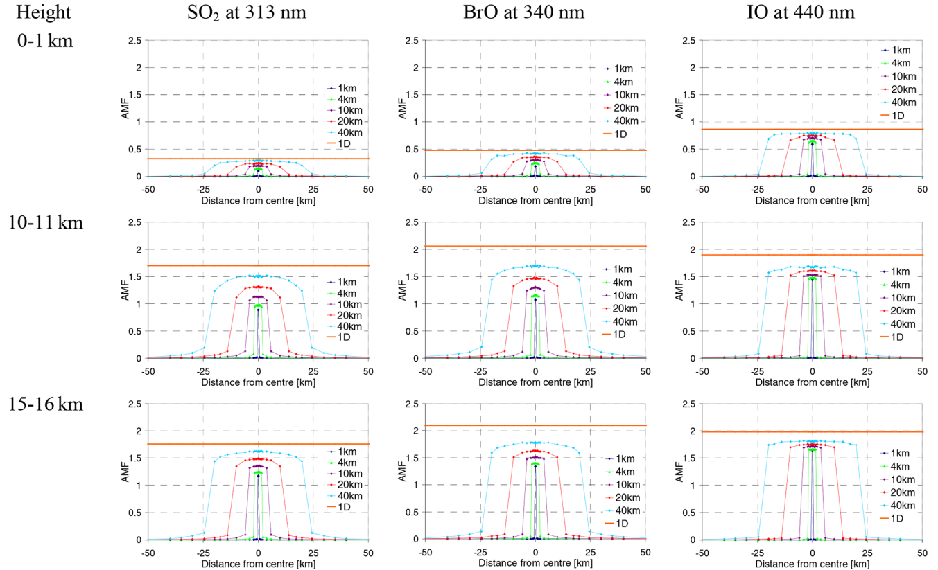
Figure C1. Same as Fig. 6 but for additional plume heights: AMFs for plume scans in near-nadir viewing geometry ( SZA = 0^\circ , VZA = 0^\circ ) at different wavelengths. It is assumed that the satellite scans the plume with a narrow FOV ( \sim 0.014^\circ ). The different colours represent AMFs for plumes with different horizontal extensions (from 1 \times 1 to 40 \times 40 \text{ km}^2 ).
