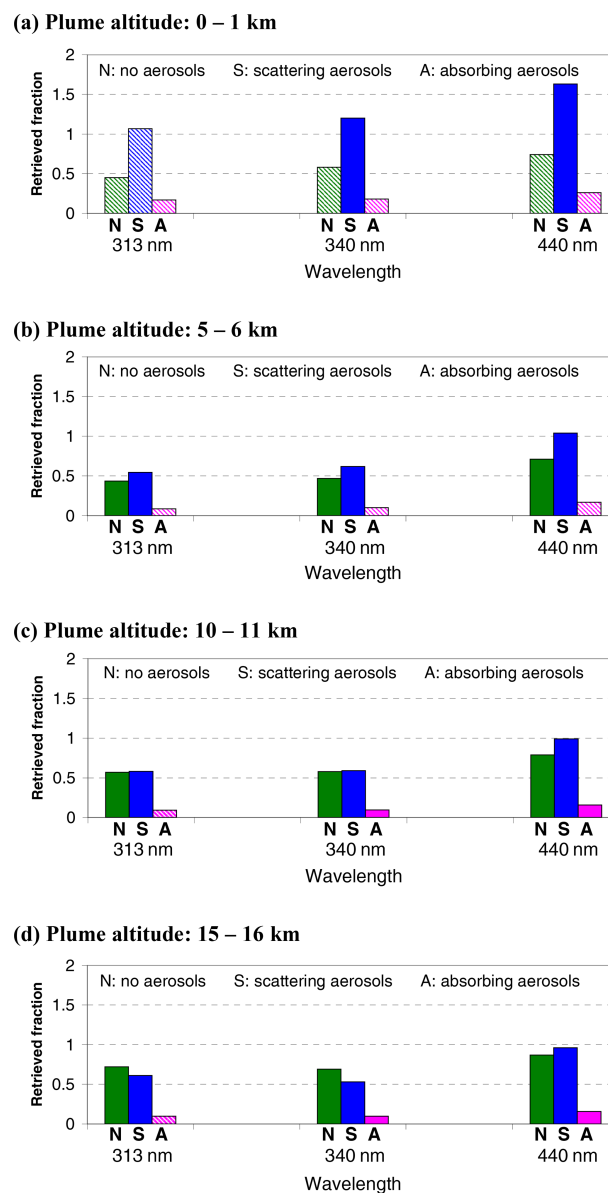
Figure 12. Retrieved fraction of the plume content at different wavelengths for different plume heights and aerosol scenarios for TROPOMI observations (horizontal plume extension 1 \times 1 \text{ km}^2 ). Hatched bars indicate scenarios for which the absorption is below the detection limit for the weak trace gas scenarios described in Sect. 2.1 (results for the satellite pixel directly above the plume).
