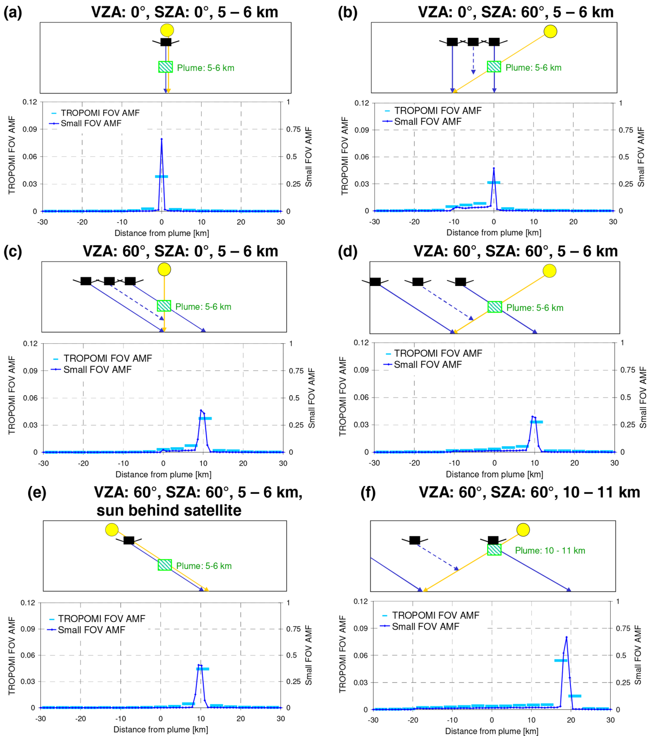
Figure E2. AMFs for TROPOMI observations of elevated plumes for different combinations of SZA and VZA. The blue lines show the AMFs for observations with a narrow FOV ( \sim 0.014^\circ ) (right y axis). The bright-blue symbols represent simulations with a TROPOMI FOV (left axis). All simulations are for BrO at 340 nm and plume sizes of 1 \times 1 \times 1 \text{ km}^3 .
