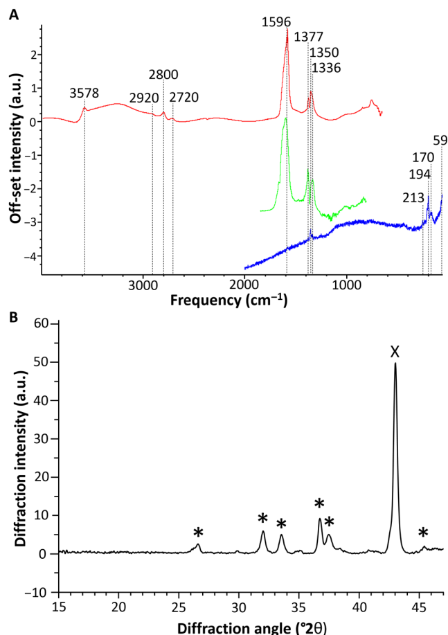
Fig. 4. Experimental spectra of basic Cu formate. (A) O-PTIR (green), SR-μFTIR (red), and μRaman (blue) on a corroded wire (sample 3W). a.u., arbitrary units. (B) XRPD collected on the corroded sequin (sample 15), average diffractogram for a 3-mm-long line in the degraded area of the sample. In evidence the diffraction peaks associated to Cu 2 (OH) 3 (HCOO) (*) (9) and high-Cu brass (X) (52).
