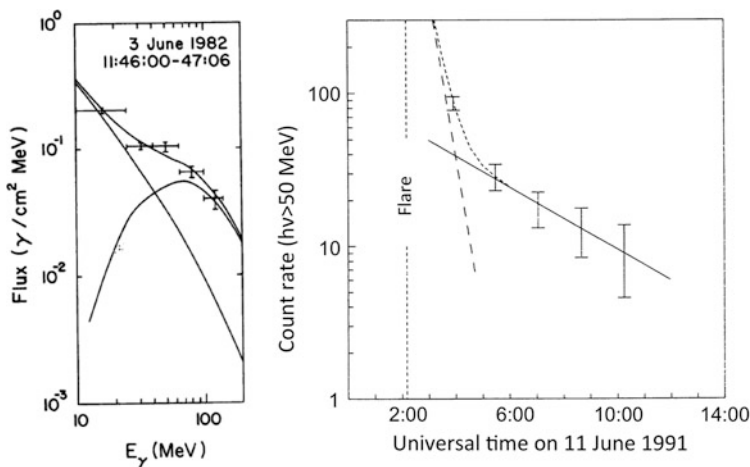
Fig. 8.1 (a) The \gamma -ray spectrum showing the pion-decay bump of the 1982 Jun 3 event, observed by SMM (Forrest et al. 1985). Credit: Forrest et al., Internat. Cosmic Ray Conf. 4, 146, 1985, courtesy W.T. Vestrand. (b) Time profile of the first sustained \gamma -ray event detected by the Compton Gamma-Ray Telescope (adapted from Kanbach et al. (1993); credit: Kanbach et al., A&A Suppl. 97, 349, 1993, reproduced with permission ©ESO)
