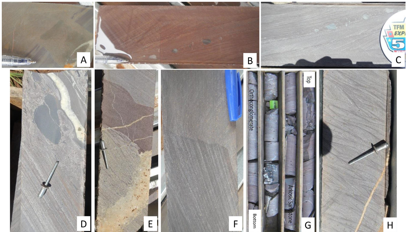
Fig. 4. Sedimentary structures and soft sediment deformation structures: (A) Neptunian dykes per descensum and sills by injection shales; (B) and (C) Scour and toll mark, (D) Balls and pillows structure, (E) Load structure, (F) Erosional surface, (G) Bouma sequence; (H) Cross bedding in arkosic sandstone.
