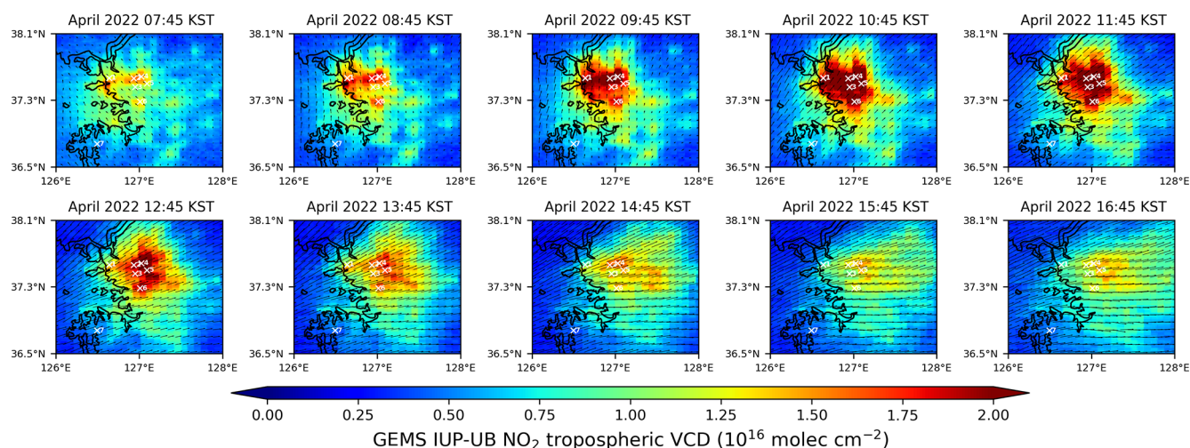
Figure A10. Maps of GEMS IUP-UB tropospheric NO 2 VCDs for the 10 observations per day averaged for April 2022 overlaid with ERA5 10 m wind data. Arrow lengths indicate wind speed, and their orientation represents wind direction. Maps show the SMA, including the sites of MAX-DOAS IUP-UB Incheon (1), Pandora Yonsei (2), Pandora Seoul (3), MAX-DOAS BIRA Seoul (4), MAX-DOAS MPIC Seoul (5), MAX-DOAS BIRA Suwon (6), and Pandora Seosan (7).
