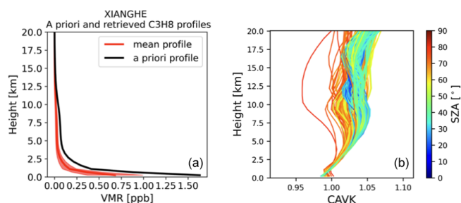
Figure 4. The a priori and retrieved C_3H_8 profiles (a) and the column averaging kernel (CAVK) varying with SZA (b).
