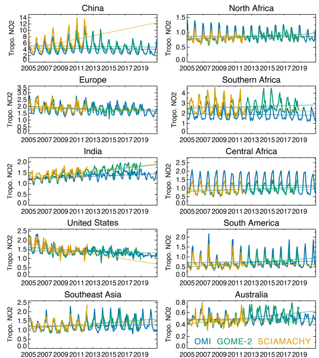
Figure 14. Time series of regional monthly mean tropospheric \text{NO}_2 columns (in 10^{15} \text{ molec. cm}^{-2} ) averaged over China ( 110\text{--}123^\circ \text{ E} , 30\text{--}40^\circ \text{ N} ), Europe ( 10^\circ \text{ W--}30^\circ \text{ E} , 35\text{--}60^\circ \text{ N} ), the US ( 70\text{--}125^\circ \text{ W} , 28\text{--}50^\circ \text{ N} ), India ( 68\text{--}89^\circ \text{ E} , 8\text{--}33^\circ \text{ N} ), South America ( 50\text{--}70^\circ \text{ W} , 20^\circ \text{ S--Equator} ), northern Africa ( 20^\circ \text{ W--}40^\circ \text{ E} , Equator– 20^\circ \text{ N} ), central Africa ( 10\text{--}40^\circ \text{ E} , Equator– 20^\circ \text{ S} ), southern Africa ( 25\text{--}34^\circ \text{ E} , 22\text{--}31^\circ \text{ S} ), southeastern Asia ( 96\text{--}105^\circ \text{ E} , 10\text{--}20^\circ \text{ N} ), and Australia ( 113\text{--}155^\circ \text{ E} , 11\text{--}44^\circ \text{ S} ) obtained from OMI (black), GOME-2 (blue), and SCIAMACHY (red).
