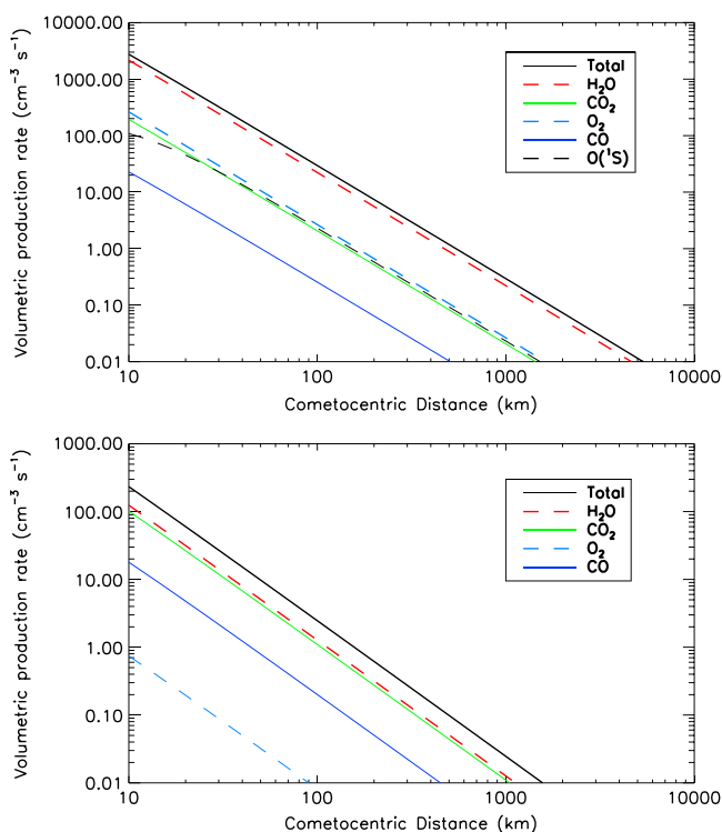
Figure 3. (top) Calculated radial profiles for the volumetric production of O(¹D) (black) from 10 to 10 4 km, along with its contribution from the photodissociation of water (red dashed line), of CO 2 (green), of O 2 (blue dashed line), and of CO (dark blue). The contribution to the O(¹D) production through radiative decay of O(¹S) is also displayed (dashed black line). (bottom) Same color code for the production of O(¹S). The radial profiles are calculated with a water production rate of 4 \times 10^{27} \text{ s}^{-1} for 25% CO, 8.3% CO 2 , and 4% of O 2 abundances relative to water at 1.35 AU heliocentric distance.
