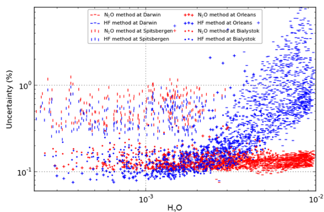
Figure 9. Relative error estimation of the tropospheric column-averaged CH 4 mole fraction using Gaussian error propagation equation for four sites, the blue corresponds to the error for the method using HF and the red to that of method using N 2 O.
