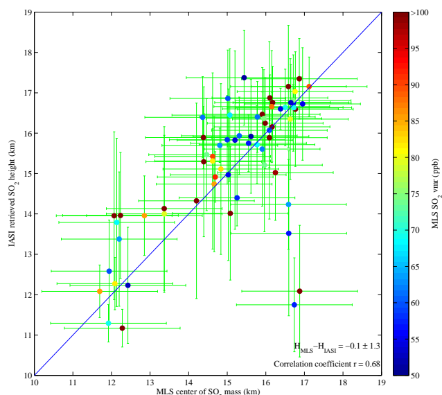
Fig. 11. Comparison of MLS centre of SO 2 mass with coincident IASI SO 2 height retrievals in a 200 km radius around the MLS measurements. The MLS errorbar was taken fixed at \pm 1.5 km, the IASI errorbar depicts the standard deviation of the coincident IASI measurements. MLS data is from the v3.3 EOS MLS Level2 which was downloaded from the NASA Goddard Space Flight Center, Data and Information Services Center ( http://disc.gsfc.nasa.gov/ ).
