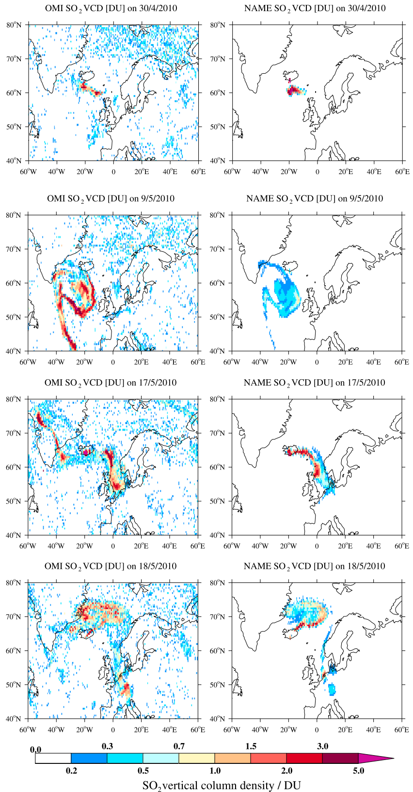
Figure 3. Comparison of the spatial distribution of SO 2 vertical column densities (VCDs in Dobson units, DU) during 4 days of the 2010 Eyjafjallajökull eruption using retrievals from the Ozone Monitoring Instrument (OMI; left) and simulated VCDs from the NAME model (right).
