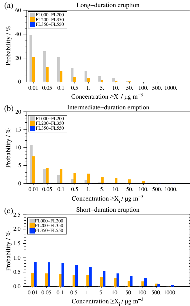
Figure 8. Mean probability (in percent) of aircraft transiting through volcanic \text{SO}_2 concentrations \geq X_i (in \mu\text{g}/\text{m}^3 ) at flight altitudes (grey = FL000-FL200; orange = FL200-FL350; blue = FL350-FL550) for 15 min or longer sampled along any of the five flight paths (shown in Figure 2) for (a) the long-duration eruption, (b) the intermediate-duration eruption, and (c) the short-duration eruption scenario. The sample space used to calculate the probabilities is defined by the analysis period considered for each eruption scenario (Table 1).
