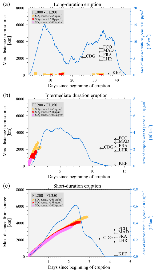
Figure 7. Maximum distance from the volcanic vent a certain threshold \text{SO}_2 mass concentration (in \mu\text{g}/\text{m}^3 ) is exceeded at flight altitudes over the course of each eruption scenario (colored stars; axis label on the left; flight altitude indicated using FL notation) for (a) the long-duration eruption at FL000-FL200, (b) the intermediate-duration eruption at FL200-FL350, and (c) the short-duration eruption at FL200-FL350. The \text{SO}_2 mass concentration thresholds are defined based on the UK Department for Environment, Food, and Rural Affairs (DEFRA) legislation and warning levels for \text{SO}_2 to protect public health [Connolly et al. , 2013]. Humans can perceive \text{SO}_2 at mixing ratios >300 ppbv [IVHNN, 2014], which is about 240 \mu\text{g}/\text{m}^3 at 11 km ( \sim 36,000 ft) altitude using the U.S. 1976 standard atmospheric profile. Also shown are the distances of European airports with respect to the volcanic vent (FCO = Fiumicino Airport, Italy; MAD = Adolfo Suárez Madrid-Barajas Airport, Spain; FRA = Frankfurt Airport, Germany; CDG = Paris Charles de Gaulle Airport, France; LHR = London Heathrow Airport, United Kingdom; KEF = Keflavik International Airport, Iceland). The solid blue line shows the area of airspace where volcanic \text{SO}_2 concentrations are greater than 0.1 \mu\text{g}/\text{m}^3 (axis label on the right; area is given in 10^6 \text{ km}^2 out of about 100 \times 10^6 \text{ km}^2 of the total area considered in the model domain) for each eruption scenario.
