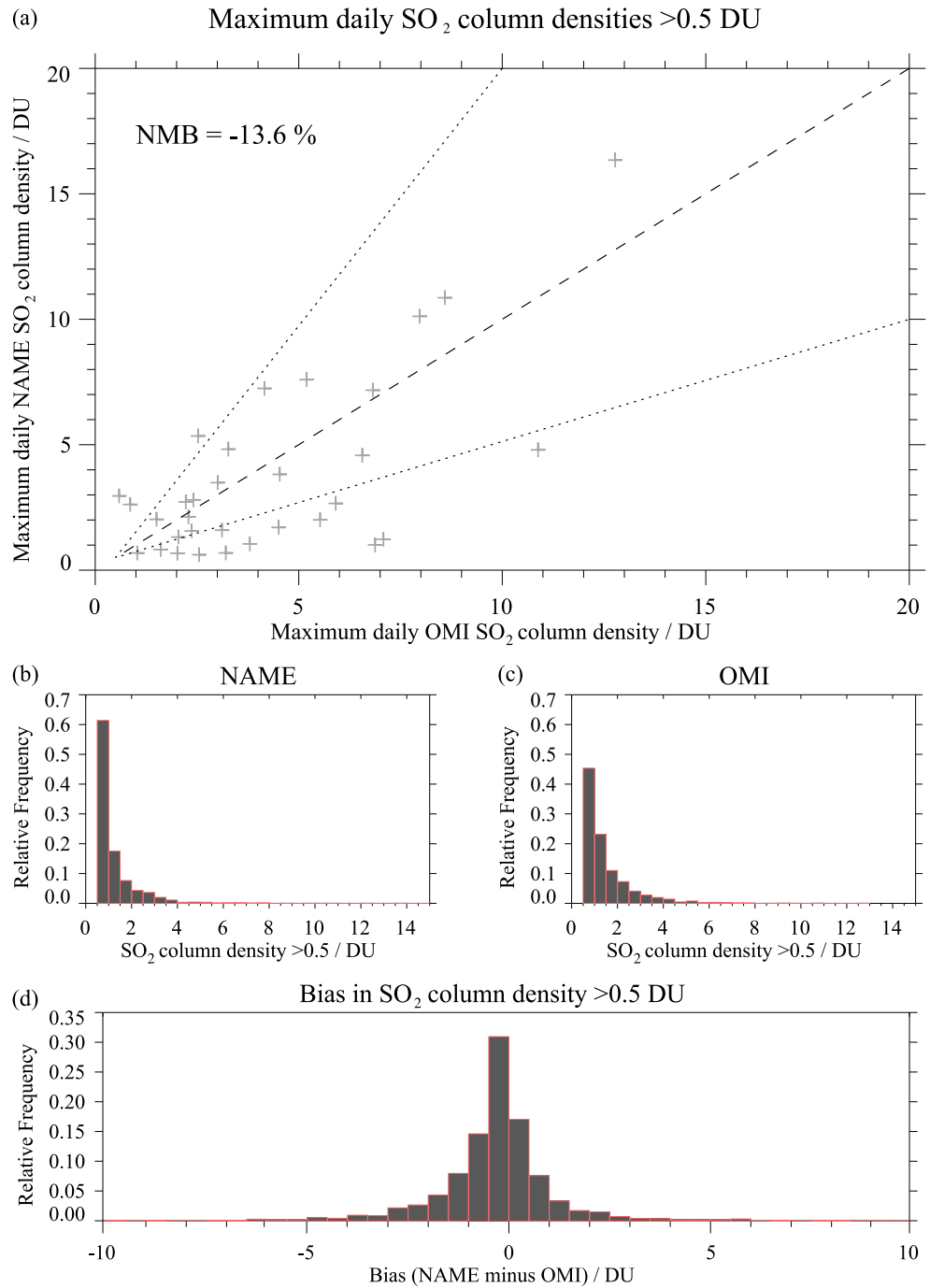
Figure 4. Comparison of (a) maximum SO 2 vertical column densities (VCDs in Dobson units, DU) greater than 0.5 DU retrieved by the Ozone Monitoring Instrument (OMI) with maximum NAME VCDs for the period 14 April to 30 May 2010 of the Eyjafjallajökull eruption. Also shown is the normalized mean bias (NMB in percent). For the comparison, the maximum was located anywhere in a given scene (i.e., maximum VCDs shown may not be spatially collocated in NAME and OMI scenes). The relative frequency distribution of all gridded SO 2 VCDs greater than 0.5 are shown (b) for NAME and (c) for OMI, and (d) The relative frequency distribution of the bias (NAME minus OMI) in SO 2 VCDs.
