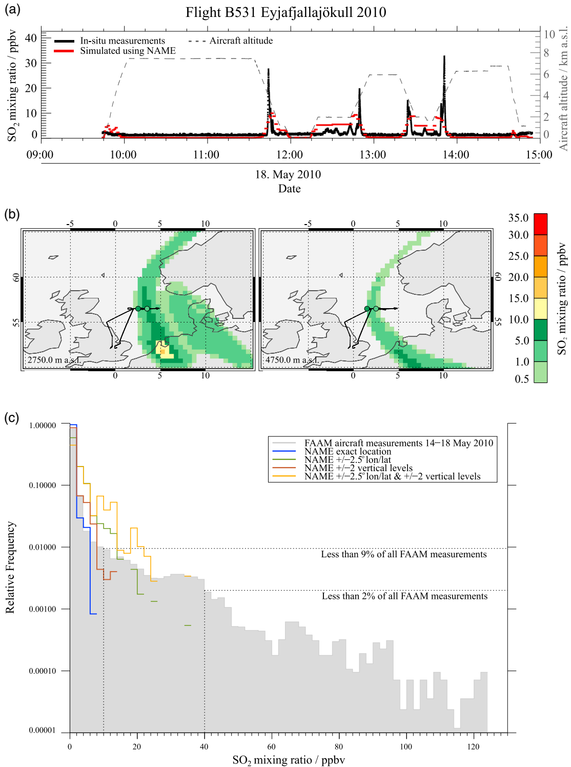
Figure 5. Comparison of SO 2 mixing ratios (in parts per billion by volume, ppbv) measured by the UK FAAM research aircraft during May 2010 to those simulated in NAME. (a) In situ measurements from FMM flight B531 (black) on 18 May 2010 with simulated (red) SO 2 mixing ratios, which are sampled along the flight track (solid black line in Figure 5b). In Figure 5a the aircraft altitude is shown by the dashed grey line. (b) A comparison of the spatial distribution of simulated SO 2 mixing ratios with in situ measurements (colored circles along flight track) on 18 May 2010. (c) The relative frequency of all aircraft measurements made in the period 14–18 May 2010 (grey) with that of simulated SO 2 mixing ratios, which have been sampled along the FAAM flight paths for the same period (colored lines). The colored lines show simulated mixing ratios obtained using different levels of model sampling tolerance with regard to the flight track (blue = exact location in terms of longitude, latitude, and height above sea level; green = maximum SO 2 mixing ratio found within ±2.5° longitude/latitude; brown = maximum SO 2 mixing ratio found within ±2 vertical output levels (±1 km); orange = maximum SO 2 mixing ratio found within ±2.5° longitude/latitude and ±2 vertical output levels).
