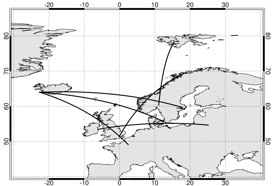
Figure 2. Map showing the five representative flight paths (black lines) that are used to calculate the probability of 15 min or longer periods that an aircraft could be exposed to volcanic sulfur dioxide. These paths are defined so that they pass through the volcanic plume of each eruption scenario.
