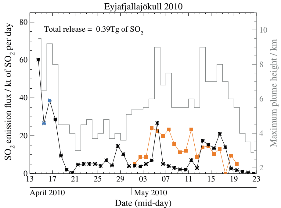
Figure 1. Daily sulfur dioxide ( \text{SO}_2 ) mass fluxes (black stars and axis labels on the left, in kilotons per day) for the 2010 Eyjafjallajökull eruption derived using the petrological method [Thordarson et al. , 2011] and daily maximum plume height (solid grey line and axis labels on the right, in kilometer above sea level) used in the model to simulate the long-duration eruption scenario. Blue stars indicate that in the model, the \text{SO}_2 mass flux was reduced to 0.1% of the petrological flux estimate in order to account for in-plume scavenging of sulfur species as observed during the early phases of Eyjafjallajökull 2010. Orange squares are \text{SO}_2 mass fluxes derived using GOME-2 retrievals in combination with inverse modeling [Flemming and Inness, 2013].
