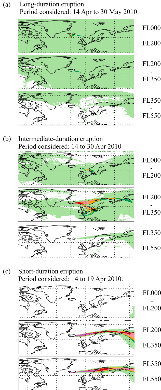
Figure 6. Spatial distribution of maximum 15 min mean SO 2 mass concentrations (in µg/m 3 ) simulated at flight altitudes at any time over a certain period of time considered for (a) the long-duration eruption, (b) the intermediate-duration eruption, and (c) the short-duration eruption scenario (see section 2 and Table 1 for details on the eruption period considered). Humans can perceive SO 2 at mixing ratios >300 ppbv [JVHNN, 2014], which is about 240 µg/m 3 at 11 km (~36,000 ft) altitude using the U.S. 1976 standard atmospheric profile. The label used for the SO 2 mass concentrations uses a similar color coding as used by the UK Department for Environment, Food, and Rural Affairs (DEFRA) for SO 2 to distinguish warning levels to protect public health [Connolly et al., 2013].
