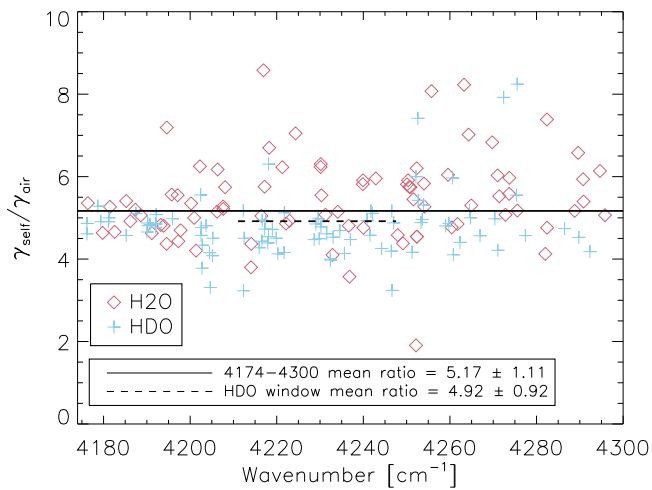
Fig. 2. Ratios between the self-broadened and air-broadened half-widths of the original Jenouvrier et al. (2007) spectroscopy. Plotted for the 174 lines with a line intensity stronger than 10^{-25} cm -1 (molecule cm -2 ) -1 . The solid and dashed lines indicate the mean ratio for the 4174–4300 cm -1 and the HDO retrieval window (4212–4248 cm -1 ), respectively.
