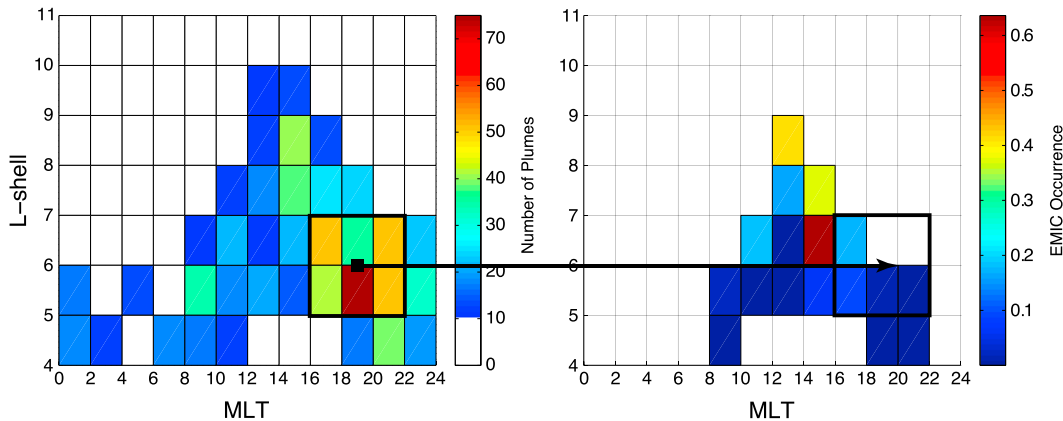
Figure 3. (left) L /MLT distribution of plasmaspheric plumets. (right) L /MLT EMIC wave occurrence rate in plumets. The black rectangle shows the region with maximum plume number. Bins with less than 10 plume crossings are not colored.
