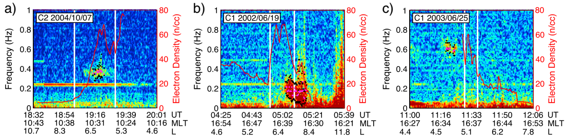
Figure 1. Spectrograms of the perpendicular component of magnetic field showing the EMIC wave location with respect to the plume: (a) inside, (b) spanning both inside and outside, and (c) outside. White vertical lines show the plume boundaries. The black and the purple dots define the EMIC bandwidth and the maximum power, respectively. The WHISPER electron density is plotted on top of the spectrograms by the red lines (where available).
