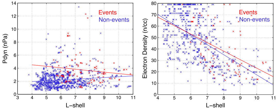
Figure 6. (left) Solar wind dynamic pressure and (right) electron density and as a function of L-shell and linear regression lines for EMIC events (red) and nonevents (blue).
