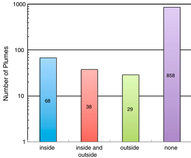
Figure 2. Distribution of EMIC wave location with respect to the plume. Note the logarithmic scale on the y axis.
