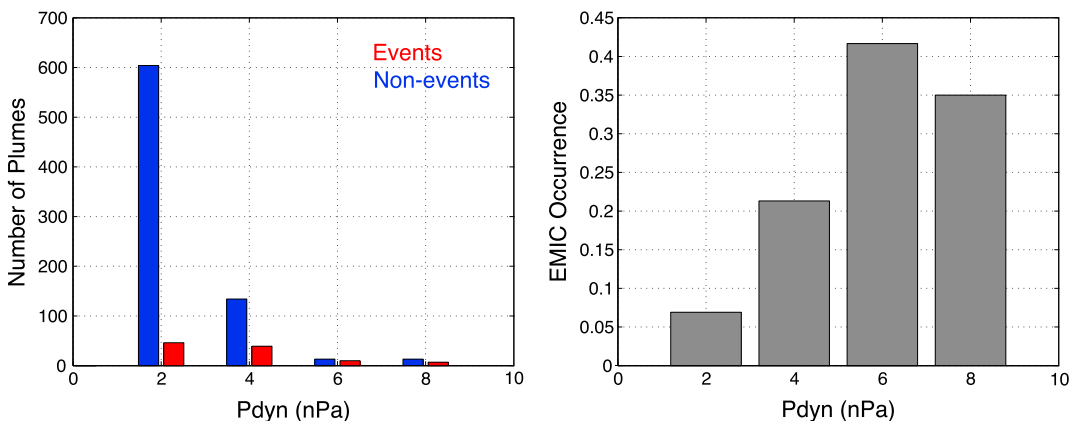
Figure 5. (left) Number of events (red) and nonevents (blue) and (right) EMIC wave occurrence rate in plumes as a function of solar wind dynamic pressure.
