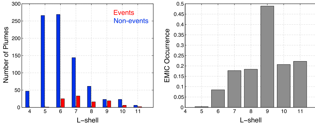
Figure 4. (left) Number of events (red) and nonevents (blue) and (right) EMIC wave occurrence rate in plumes as a function of L-shell.
