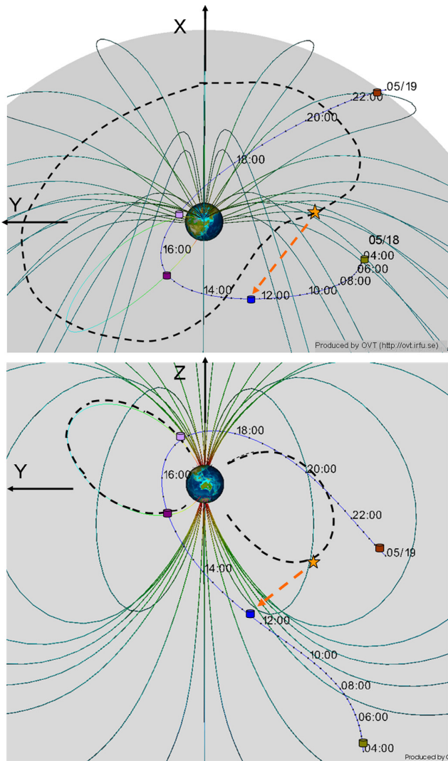
Fig. 11. Views in GSM coordinate system from OVT (Orbit Visualization Tool, http://ovt.irfu.se ). C3–C4 orbit on 18 May 2008, and magnetopause field lines are projected onto X – Y plane (top) and Y – Z plane (bottom). The NTC source is indicated by a star; the observing point at 12:20 UTC by a blue symbol; other positions of the (C3–C4) pair by symbols in various colours. Plasmopause crossings, occurring at 15:20 UTC and 16:50 UTC in the dusk sector, are shown in dark and light purple. Magnetopause crossings, occurring at 04:20 UTC and 23:30 UTC, are shown in light green and brown. Dashed curves sketch possible positions of plasmopause, equatorial boundary in upper panel, selected magnetic flux tubes along plasmopause surface in lower panel.
