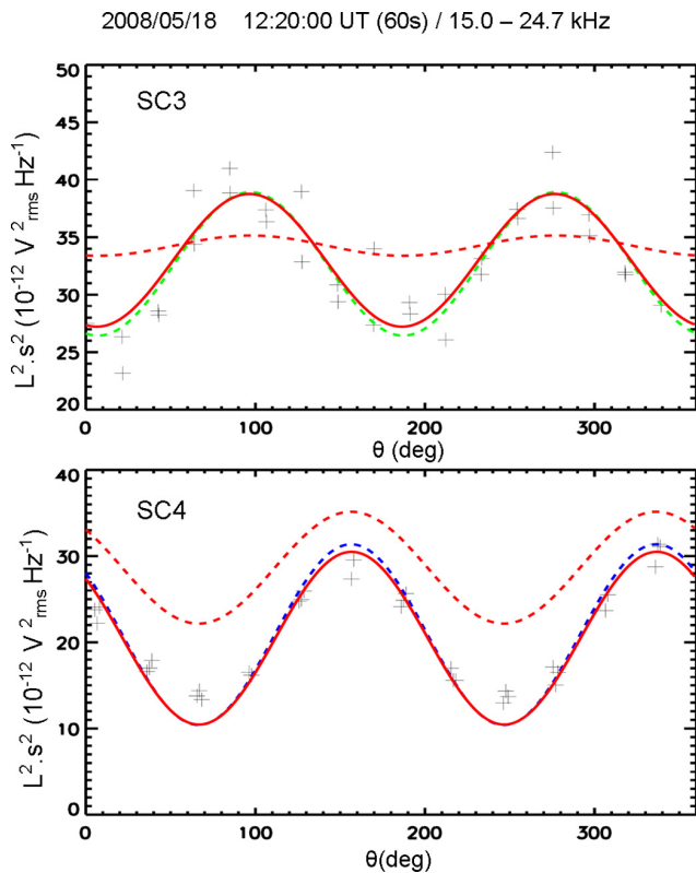
Fig. 4. Electric signal versus antenna attitudes, with C3 data at top and C4 data at bottom (same data set as in Fig. 1). As in Fig. 1, grey crosses are measured samples, the dashed green curve (top) and dashed blue curve (bottom) represent best fits to instantaneous signal variations. Red curves correspond to the modelled electric fields (instantaneous power variations) solution of the DSM tool under respectively elliptical polarization assumption (solid lines) and circular polarization assumption (dashed lines).
