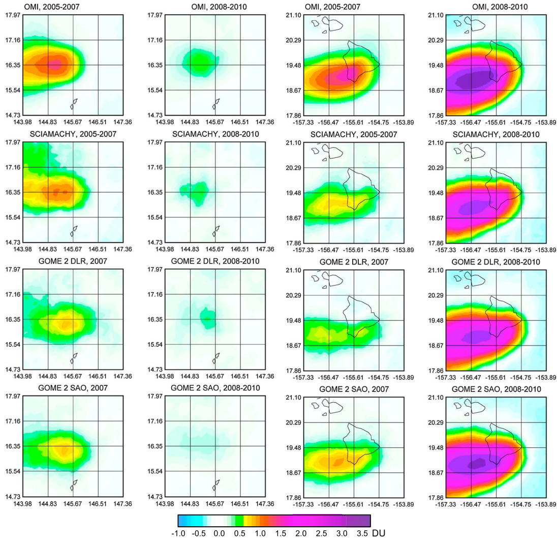
Figure 3. Mean SO 2 distribution over Anatahan and Kilauea volcanoes in DU smoothed using the averaging radius of 60 km for two time intervals. All four data products can successfully track changes in emissions from individual volcanoes. Note that a cutoff limit of 15 DU was used to remove impacts of large eruptions.
