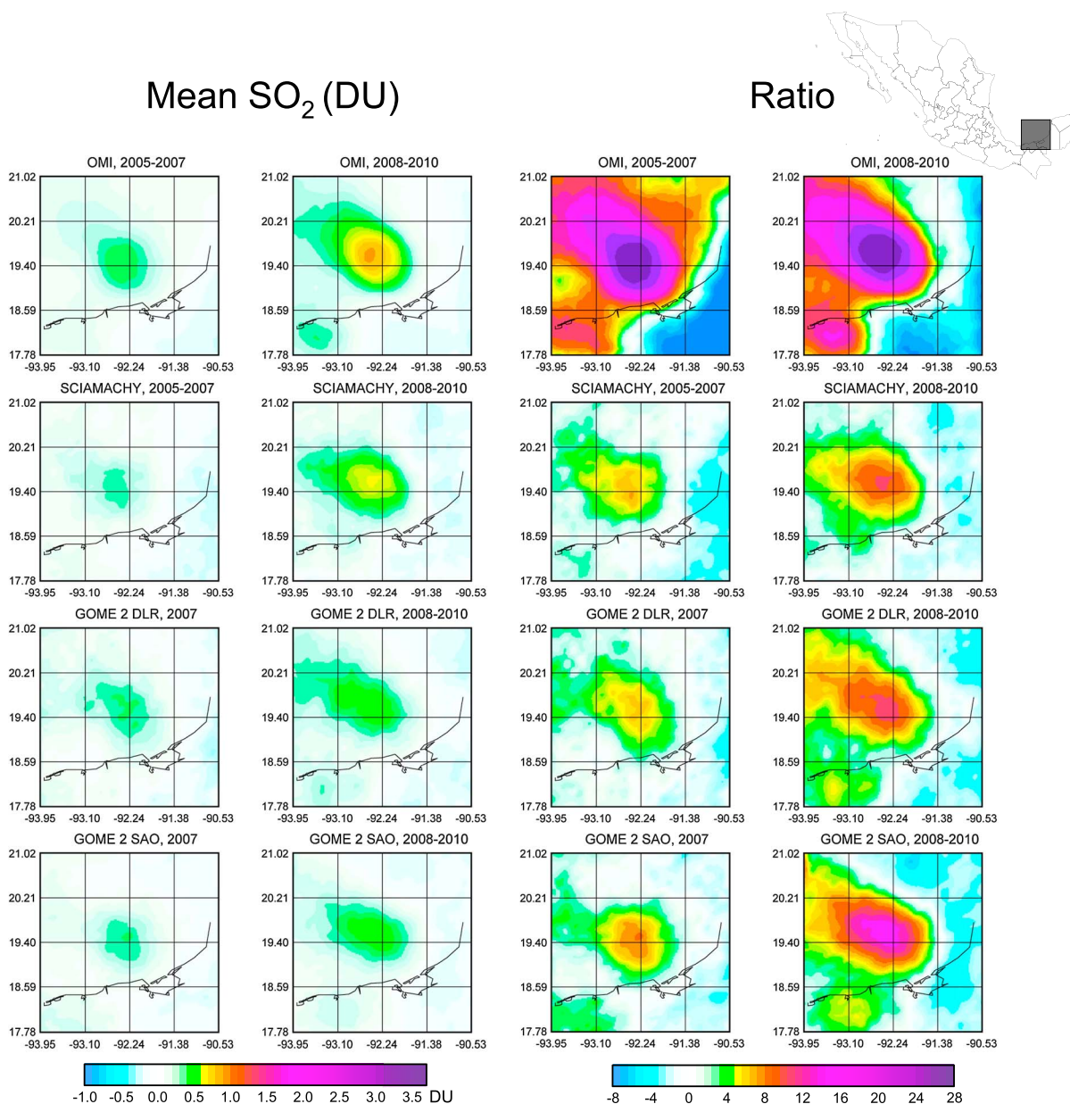
Figure 4. Mean SO 2 distribution over Cantarell and Ku-Maloob-Zaap Oil Fields, Gulf of Mexico, for 2005–2007 and 2008–2010. Data are smoothed using the averaging radius of 60 km. SO 2 values in DU and the ratios between the mean SO 2 and the standard error of the mean are shown.
