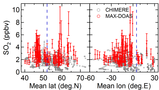
Fig. 15. \text{SO}_2 VMRs from MAX-DOAS (red) and CHIMERE (gray) plotted against mean latitude and longitude of the 10-day back trajectories. Error bars represent the error range of MAX-DOAS \text{SO}_2 VMR data. The location of Cabauw is indicated by vertical dashed lines.
