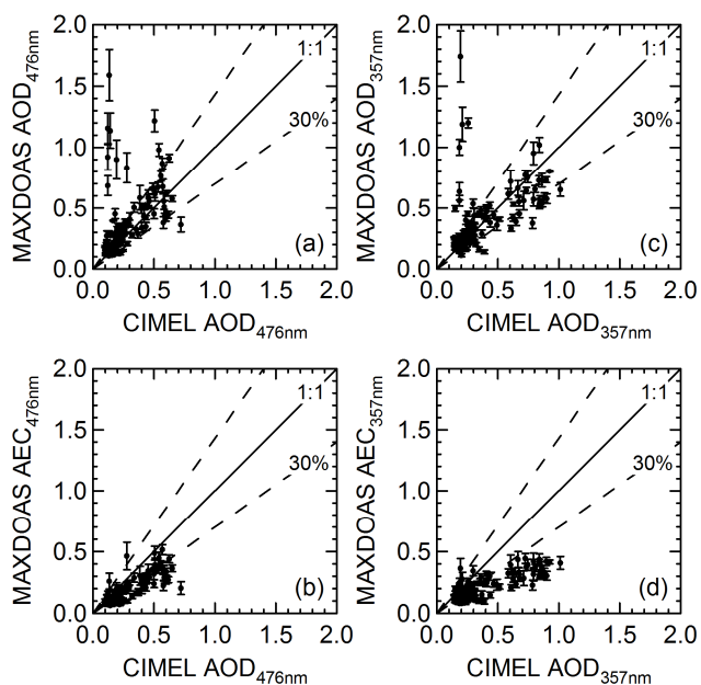
Fig. 6. Correlations between MAX-DOAS aerosol products (AOD and AEC at 0–1 km) and CIMEL sunphotometer AOD data. Correlations for 476 nm (a and b) and 357 nm (c and d) are plotted.
