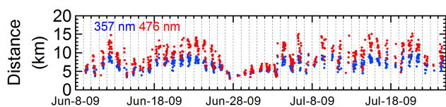
Fig. 17. Horizontal distances ( D ) of air masses measured by MAX-DOAS for the 0–1 km layer. D values at 357 and 476 nm are shown in blue and red, respectively.
