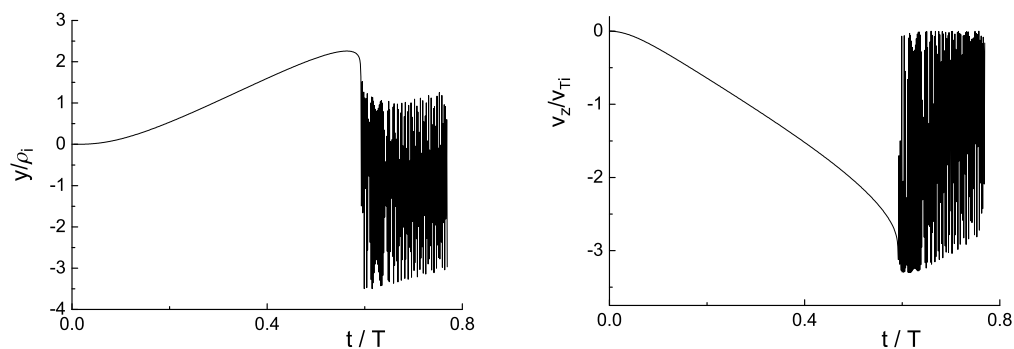
Figure 1: Left: displacement y(t)[=v_x(t)/\Omega] normalized to the ion gyro-radius \rho_i , showing stochastic behavior within one wave-period T , for a tokamak plasma. Right: particle velocity v_z(t) along the magnetic field for a tokamak plasma, normalized to the ion thermal speed, corresponding to the displacement from the figure left.
