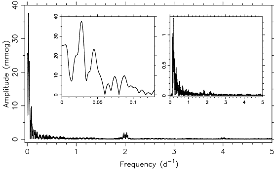
Fig. 3. Amplitude spectrum of the CoRoT data of HD 50064, up to 5 \text{ d}^{-1} ( 57.87 \mu\text{Hz} ). At higher frequencies, only harmonics of the satellite orbit of 6184 s occur, with an amplitude below 1 mmag. The insets show an enlarged section at low frequencies ( left ) and the amplitude spectrum of the residuals after prewhitening with the dominant frequency and six of its (sub)harmonics ( right ).
