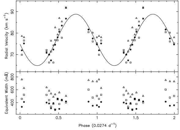
Fig. 4. Phase diagrams of the radial velocity and equivalent width of the three spectral lines He I 4471 Å (squares), He I 6678 Å (triangles), and Mg II 4481 Å (filled dots). Each measurement occurs twice for visibility purposes.
