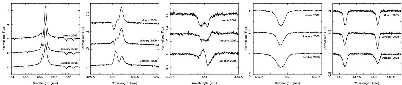
Fig. 2. Average profiles at three epochs of H, He, and an Mg line of HD 50064 (from left to right: H\alpha , H\beta , H\gamma , He I at 6678 Å, and He I at 4471 Å, as well as Mg II at 4481 Å).
