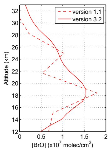
Fig. 1. Comparison between versions 1.1 and 3.2 of SCIAMACHY limb BrO profiles for 5 May 2003 close to Harestua (latitude and longitude at the tangent point: 62.3° N and 13.9° E, respectively). The SZA at tangent point is about 42° and the orbit and state numbers are 6531 and 27 (NRT Level 0 file n°442) for version 1.1 profile and 6532 and 11 for version 3.2 profile.
