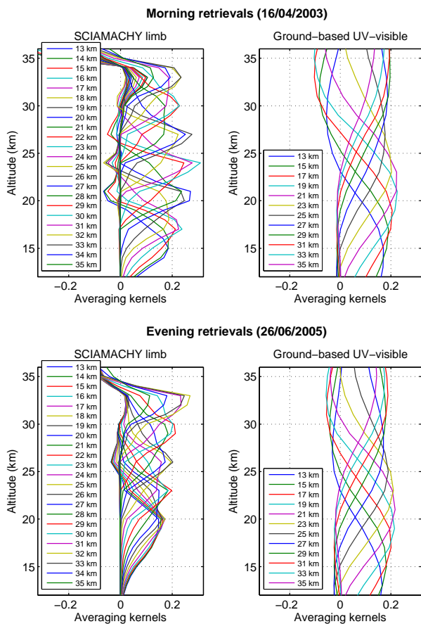
Fig. 2. Typical examples of averaging kernels for morning (upper plots) and evening (lower plots) SCIAMACHY limb and ground-based UV-visible BrO retrievals. They correspond to the Harestua 16 April 2003 morning and 26 June 2005 evening retrievals.
