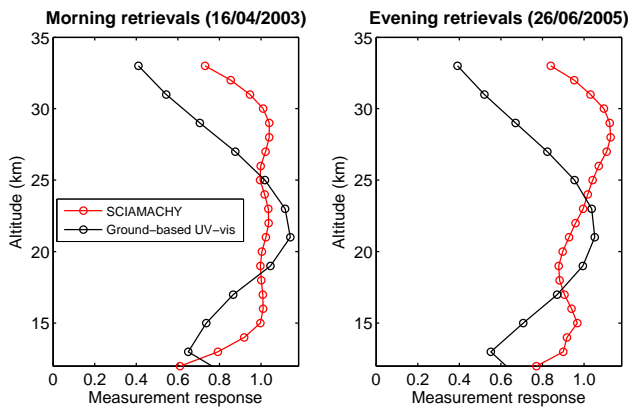
Fig. 3. Typical examples of measurement response functions for morning (left plot) and evening (right plot) SCIAMACHY limb and ground-based UV-visible BrO retrievals. They correspond to the Harestua 16 April 2003 morning and 26 June 2005 evening retrievals.
