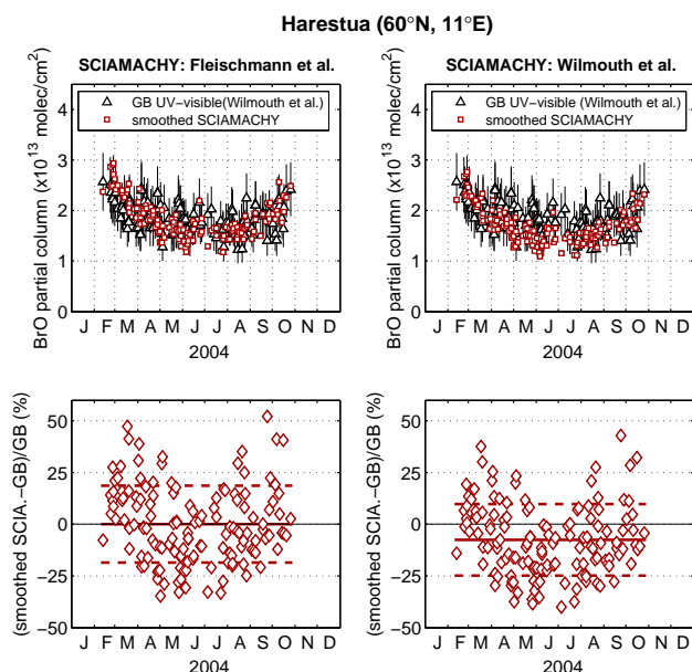
Fig. 13. Comparison of the 15–27 km BrO partial columns for the year 2004 at Harestua using the standard retrieval settings (left plots) and the same Wilmouth et al. (1999) BrO cross sections in both SCIAMACHY and ground-based retrievals (right plots). The relative differences appear in the lower plots. The error bars on the ground-based data correspond to the total error (systematic error + total retrieval error), estimated as in Hendrick et al. (2007). The solid and dashed red lines in the lower plots correspond to the mean relative difference and its one-sigma standard deviation, respectively.
