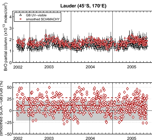
Fig. 7. Comparison of the 15–27 km BrO partial columns calculated from the smoothed SCIAMACHY limb and ground-based UV-visible profiles at Lauder (45° S, 170° E) for the 2002–2005 period (morning coincidences). The relative differences appear on the lower plot. The error bars on the ground-based data correspond to the total error (systematic error + total retrieval error), estimated as in Hendrick et al. (2007). The solid and dashed red lines in the lower plot correspond to the mean relative difference and its one-sigma standard deviation, respectively. The grey-shaded area indicates the mean uncertainty region for the ground-based UV-visible partial columns.
