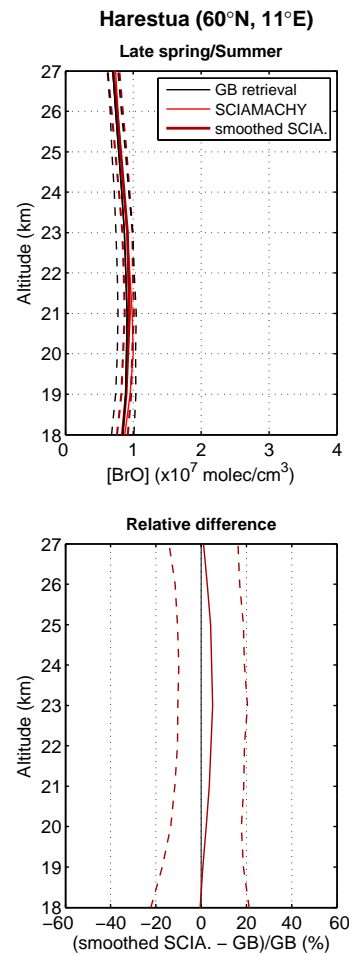
Fig. 10. Comparison between mean SCIAMACHY limb (thin red and thick dark red solid lines) and ground-based UV-visible BrO profiles (solid black line) at Harestua (60° N, 11° E) for evening conditions for the 2002–2006 period (49 coincidences). The mean relative differences appear in the lower plot. They have been plotted for the smoothed SCIAMACHY profile. In both plots, the dashed lines represent the one-sigma standard deviation. The standard deviation of the unsmoothed SCIAMACHY profile is similar to the one calculated for the smoothed profile.
