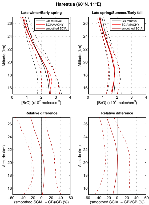
Fig. 9. Comparison between mean SCIAMACHY limb (thin red and thick dark red solid lines) and ground-based UV-visible BrO profiles (solid black line) at Harestua (60° N, 11° E) for the 2002–2006 period (morning coincidences). Profiles have been plotted separately for late winter/early spring (left plot) and late spring/summer/early fall (right plot) conditions. The number of coincident events is 154 and 358, respectively. The mean relative differences appear in the lower plots. They have been plotted for the smoothed SCIAMACHY profiles. In the four plots, the dashed lines represent the one-sigma standard deviation. The standard deviation of the unsmoothed SCIAMACHY profiles is similar to the one calculated for the smoothed profiles.
