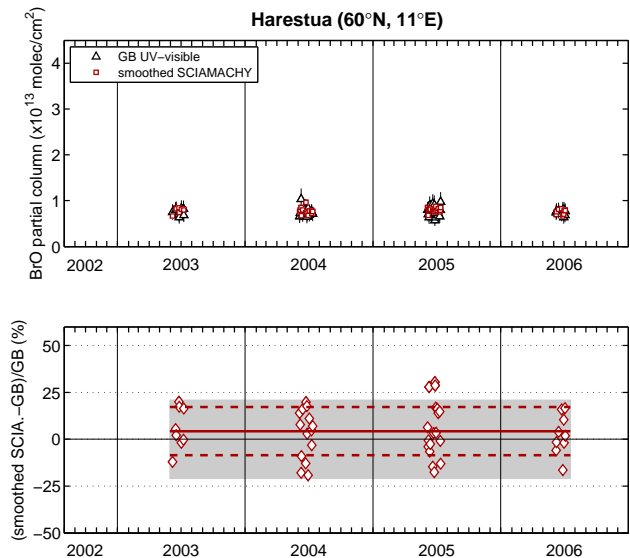
Fig. 12. Comparison of the 18–27 km BrO partial columns calculated from the smoothed SCIAMACHY limb and ground-based UV-visible profiles at Harestua (60° N, 11° E) for the 2002–2006 period (evening coincidences). The relative differences appear on the lower plot. The error bars on the ground-based data correspond to the total error (systematic error + total retrieval error), estimated as in Hendrick et al. (2007). The solid and dashed red lines in the lower plot correspond to the mean relative difference and its one-sigma standard deviation, respectively. The grey-shaded area indicates the mean uncertainty region for the ground-based UV-visible partial columns.
