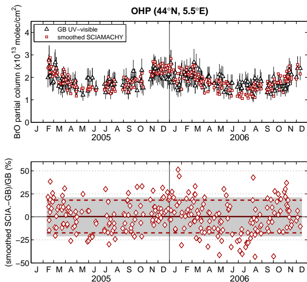
Fig. 6. Comparison of the 15–27 km BrO partial columns calculated from the smoothed SCIAMACHY limb and ground-based UV-visible profiles at OHP (44° N, 5.5° E) for the 2005–2006 period (morning coincidences). The relative differences appear on the lower plot. The error bars on the ground-based data correspond to the total error (systematic error + total retrieval error), estimated as in Hendrick et al. (2007). The solid and dashed red lines in the lower plot correspond to the mean relative difference and its one-sigma standard deviation, respectively. The grey-shaded area indicates the mean uncertainty region for the ground-based UV-visible partial columns.
