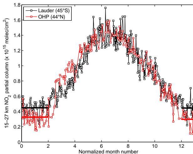
Fig. 8. Typical 15–27 km \text{NO}_2 partial column seasonal cycle at Lauder (45° S, 170° E) and OHP (44° N, 5.5° E) derived from SCIAMACHY limb profiles. At Lauder, month 0 corresponds to June 2003 and month 12 to June 2004. At OHP, month 0 corresponds to December 2005 and month 12 to December 2006. Thick solid lines correspond to mean partial columns for the months 0–2 and month 12 periods (red OHP; black: Lauder).
