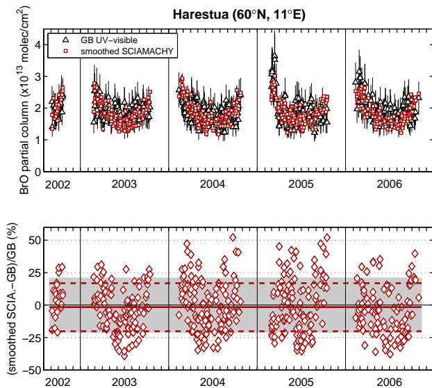
Fig. 11. Comparison of the 15–27 km BrO partial columns calculated from the smoothed SCIAMACHY limb and ground-based UV-visible profiles at Harestua (60° N, 11° E) for the 2002–2006 period (morning coincidences). The relative differences appear on the lower plot. The error bars on the ground-based data correspond to the total error (systematic error + total retrieval error), estimated as in Hendrick et al. (2007). The solid and dashed red lines in the lower plot correspond to the mean relative difference and its one-sigma standard deviation, respectively. The grey-shaded area indicates the mean uncertainty region for the ground-based UV-visible partial columns.
