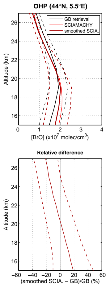
Fig. 4. Comparison between mean SCIAMACHY limb (thin red and thick dark red solid lines) and ground-based UV-visible BrO profiles (solid black line) at OHP (44° N, 5.5° E) for morning conditions for the 2005–2006 period (265 coincidences). The mean relative differences appear in the lower plot. They have been plotted for the smoothed SCIAMACHY profile. In both plots, the dashed lines represent the one-sigma standard deviation. The standard deviation of the unsmoothed SCIAMACHY profile is similar to the one calculated for the smoothed profile.
