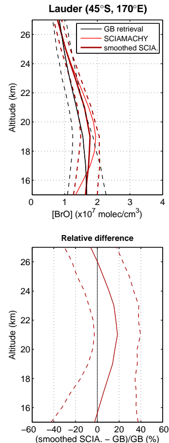
Fig. 5. Comparison between mean SCIAMACHY limb (thin red and thick dark red solid lines) and ground-based UV-visible BrO profiles (solid black line) at Lauder (45° S, 170° E) for morning conditions for the 2002–2005 period (517 coincidences). The mean relative differences appear in the lower plot. They have been plotted for the smoothed SCIAMACHY profile. In both plots, the dashed lines represent the one-sigma standard deviation. The standard deviation of the unsmoothed SCIAMACHY profile is similar to the one calculated for the smoothed profile.
