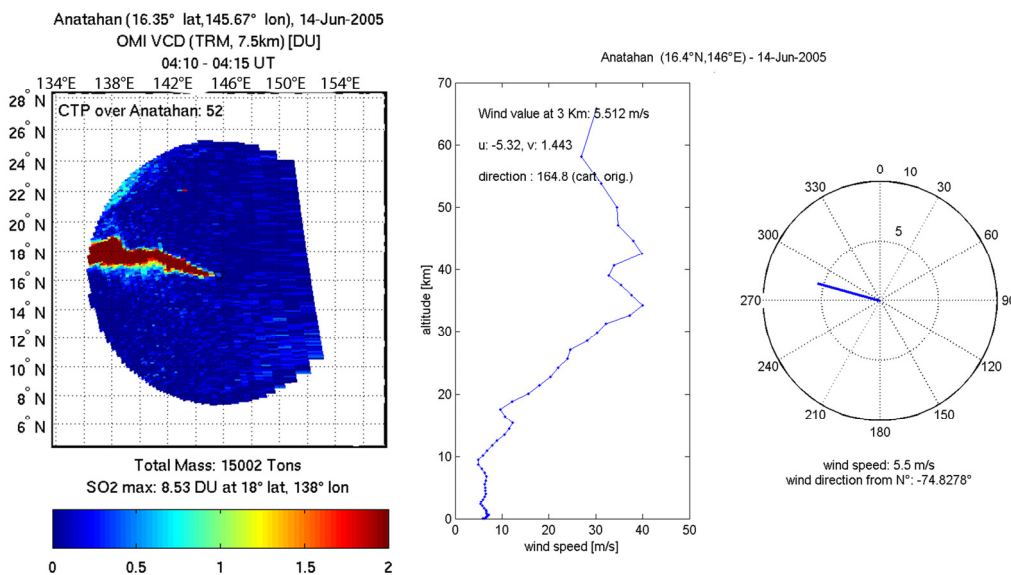
Figure 8: Maps of the SO 2 plume distribution over Anatahan on 14 June 2005 as seen by OMI on the left panel, and ECMWF wind speed and direction over the volcano on the right panel.
