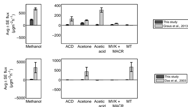
Figure 2. Comparison of BVOC exchanges at LTO with other maize studies. For comparison with Graus et al. (2013): R1 stage, 28^{\circ}\text{C} \leq T^{\circ} \leq 32^{\circ}\text{C} ; \text{PPFD} \geq 1000 \mu\text{mol m}^{-2} \text{s}^{-1} . BVOC exchanges reported by Graus et al. (2013) were up-scaled with LAI measured at LTO during the R1 stage ( 4.86 \text{ m}^2 \text{ m}^{-2} ). For comparison with Das et al. (2003): L and S stages, 24^{\circ}\text{C} \leq T^{\circ} \leq 28^{\circ}\text{C} , fluxes taken from 10:30 to 13:30 UTC in order to capture midday fluxes. See Table 1 for compound abbreviations and Table 4 for maize studies description. Note the varying scales for the y axes.
