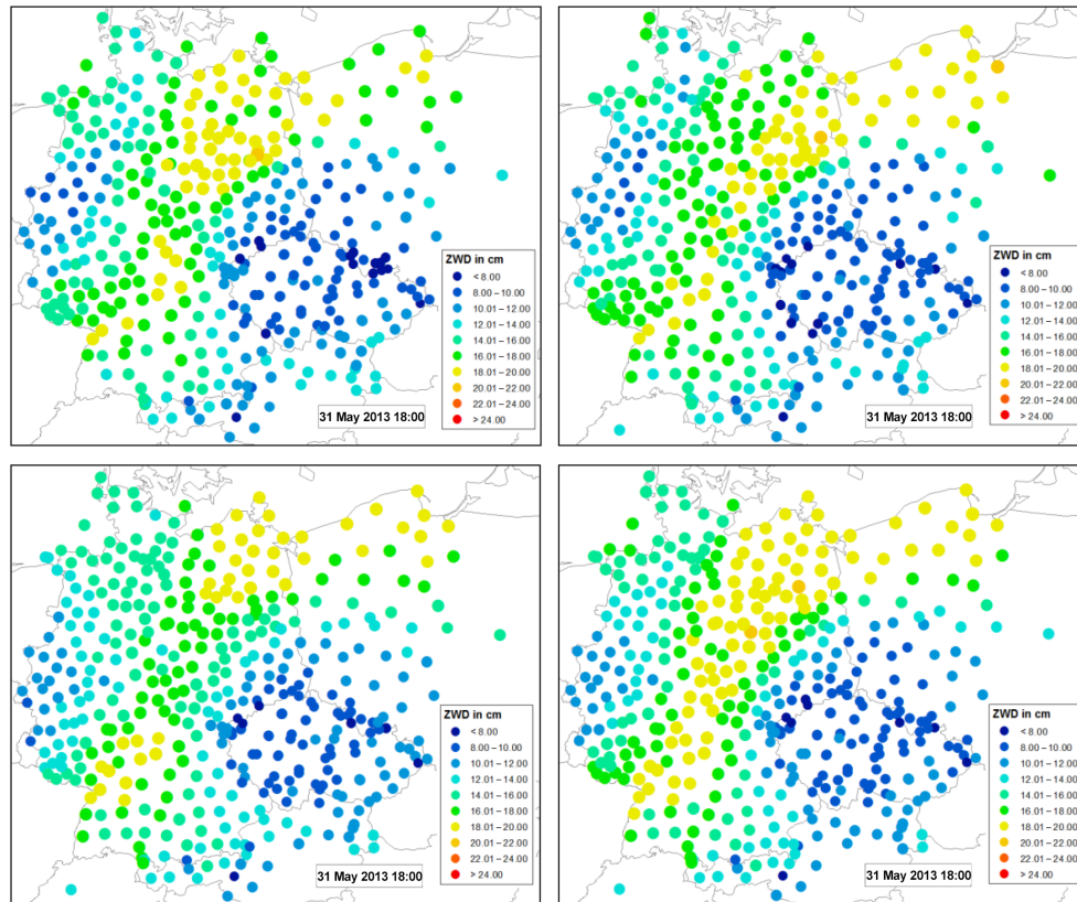
Figure 9. Fields of zenith wet delays estimated for all stations from GNSS processing (top left), ALADIN-CZ model (top right), ERA-INTERIM model (bottom left) and GFS model (bottom right) on 31 May 2013 (18:00 UTC).
