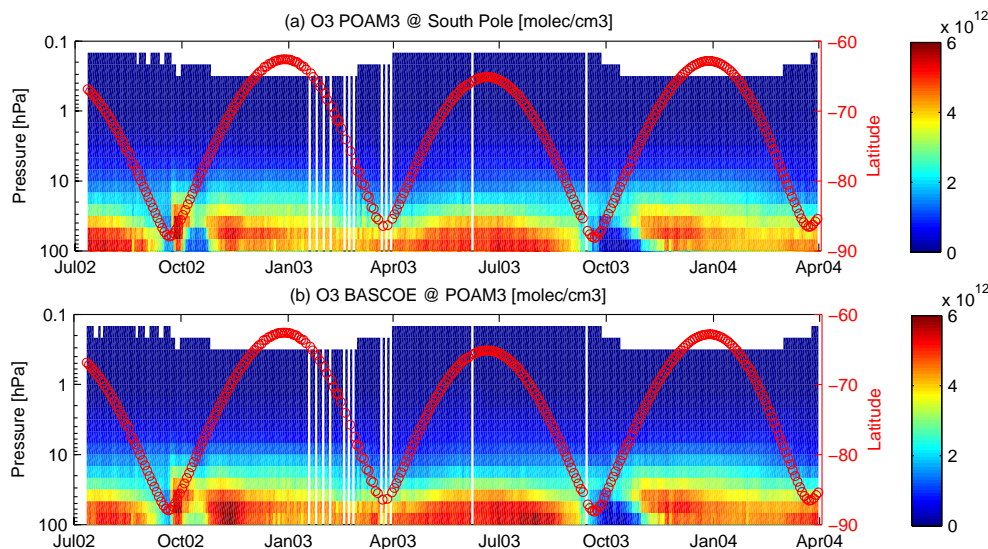
Fig. 6. Time series of POAM-III averaged over two days for ozone at South Pole (top), BASCOE ozone analyses at POAM-III (bottom), units of molec/cm 3 . Red circles correspond to the average latitude of POAM-III observations (right y-axis).
