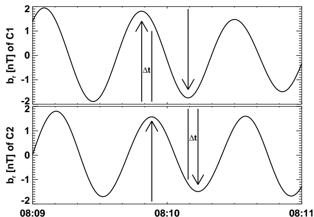
Fig. 8. Time series of the radial magnetic field oscillation of spacecraft C1 and C2.
