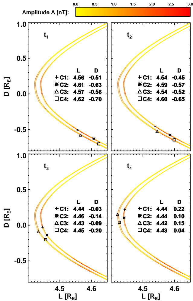
Fig. 6. Cluster orbits in L-D coordinates at t_1-t_4 . The spacecraft move from negative to positive D values across the magnetic equator ( D=0 R_E ). The color index gives the instantaneous amplitude of the transverse magnetic field oscillation.
