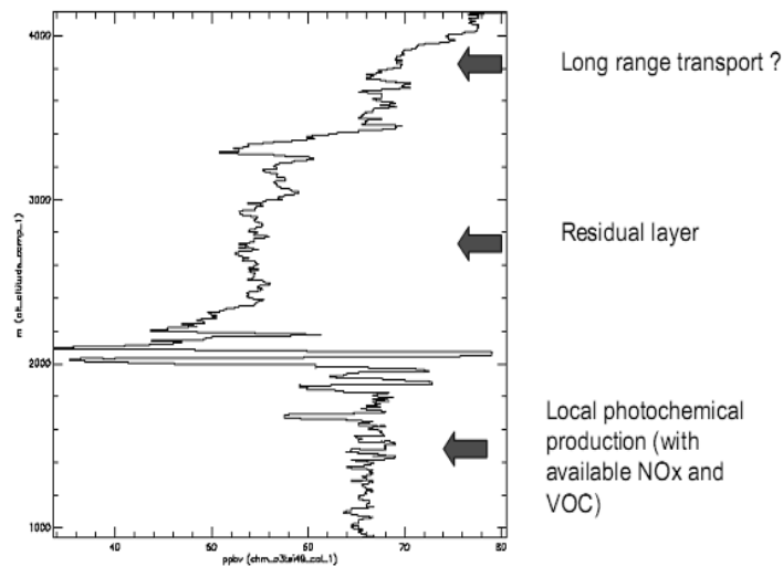
Fig. 8- Ozone distribution above IASI
