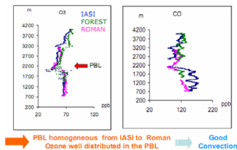
Fig. 7- Ozone and CO profiles for the 3 soundings above Iasi, forest area and Roman
