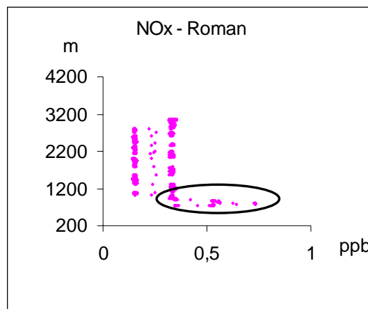
Fig. 3 - No x concentration profiles above Roman
