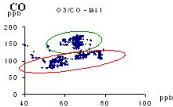
Fig. 10 - CO vs. O 3 concentrations above Iasi
