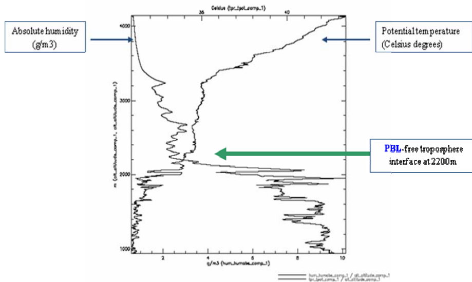
Fig. 5 - Potential temperature and absolute humidity profiles above Iasi during the flight
