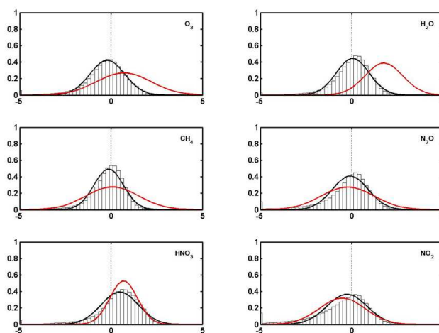
Fig. 2. Evaluation of analyses using histograms of OmF differences (normalized by the observation error) averaged for the stratosphere, the globe and August 2003 for six stratospheric constituents: \text{O}_3 (top left), \text{H}_2\text{O} (top right), \text{CH}_4 (middle left), \text{N}_2\text{O} (middle right), \text{HNO}_3 (bottom left) and \text{NO}_2 (bottom right). The constituent observations are from ESA MIPAS off-line retrievals. The frequency of the histograms is normalized by the observations, so that the sum of the histogram values is 1. The black line is a Gaussian fit to the histograms; the red line is a Gaussian fit from a model run without assimilation. The results support the assumption of Gaussian errors in the observations and the forecast, and show the analyses are closer to the observations than simulations from the model run without assimilation. The experiments were performed at BIRA-IASB ( http://www.bascoe.oma.be ).
