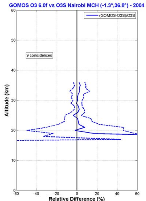
Figure 10. Same as Fig. 9 but with Kenyan NDACC station of Nairobi ozonesondes data.
