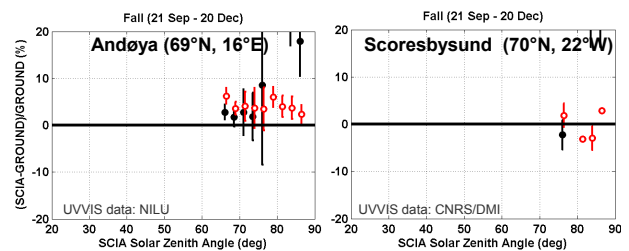
Figure 8 - Same as Fig. 7, but with UUVVIS data in fall at Andøya (Norway) and Scoresbysund (Eastern Greenland).
