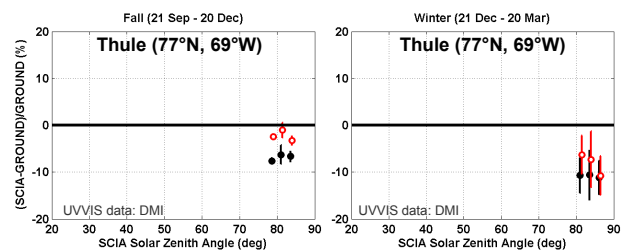
Figure 9 – Same as Fig. 7, but with UUVVIS data in fall (left) and winter (right) at Thule (Western Greenland).
