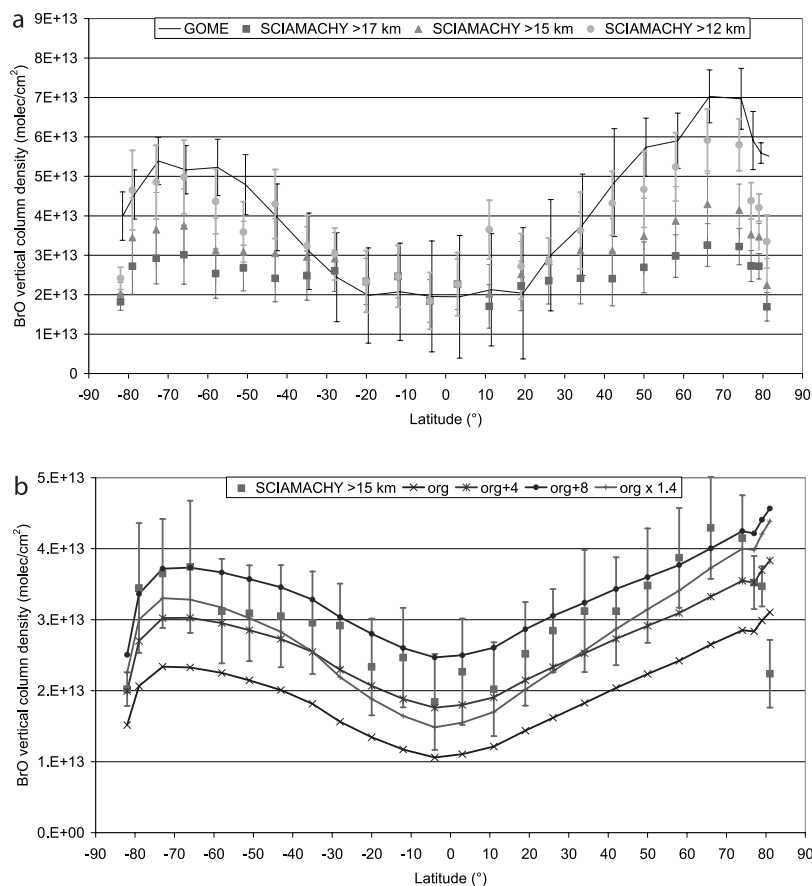
Figure 12. (a) Comparison of BrO vertical columns observed on 6 March 2003 from SCIAMACHY limb scatter and by GOME [Van Roozendaal et al. , 2002] during coincident orbits. (b) Model [McLinden et al. , 2000] BrO columns >15 km using the Wamsley et al. [1998] organic Br y versus tracer relations (updated to March 2003, see Appendix B), and with 4 and 8 pptv Br y offsets starting at 15 km. The effect of a 41% increase at all altitudes to the organic Br y profile is labeled “org × 1.4” (see text). These simulations are appropriate to SCIAMACHY local time and latitudinal sampling during orbit 5299.
