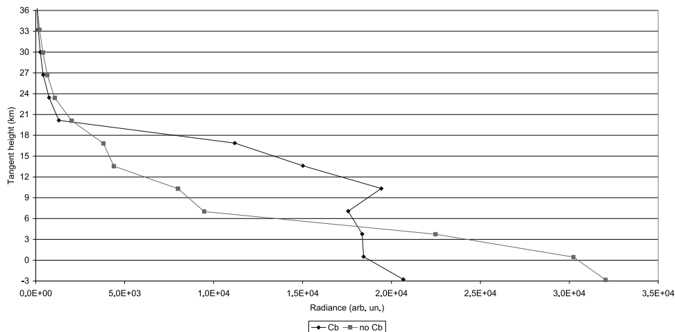
Figure 2. Limb radiance profile at \sim 1.2 \mu\text{m} observed at 20°S, 38°W in the presence of towering cumulonimbus (Cb) and at 4°N, 44°E (over arid Somalia) in the absence of such clouds on 6 March 2003.
