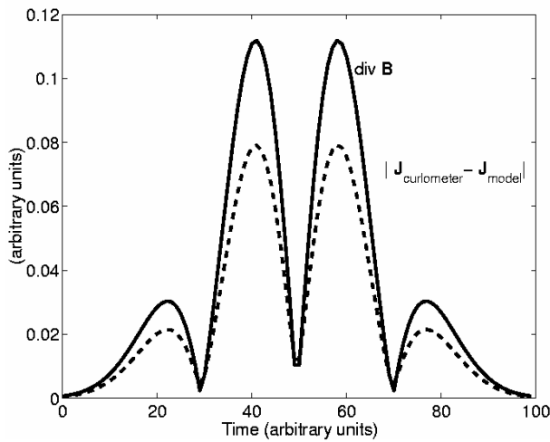
Figure 1: (a) Summary of the curlometer calculation (see also [17,18]), (b) Sample comparison between the error in the linear curlometer estimate and the linear estimate of \text{div}(\mathbf{B}) for a simple current sheet.
