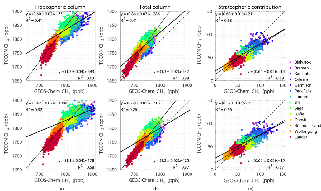
Figure 4. Daily median TCCON and smoothed daily mean GEOS-Chem base (top) and aseasional (bottom) DMFs for (a) X_{\text{CH}_4}^t , (b) X_{\text{CH}_4} , and (c) stratospheric contribution. Site colors are as in Fig. 1. Northern Hemisphere least squares regression equations are in the top left, and Southern Hemisphere least squares regression equations are in the bottom right of each plot. Dashed lines mark the one-to-one lines.
