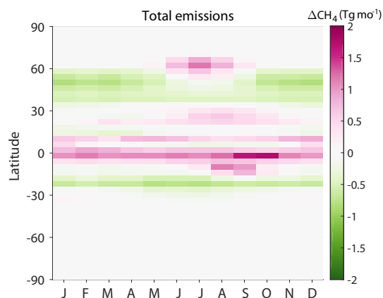
Figure B1. Monthly averages of the difference in total CH 4 emissions between the base and aseasonal GEOS-Chem simulations, summed over each zonal band, in Tg mo -1 .
