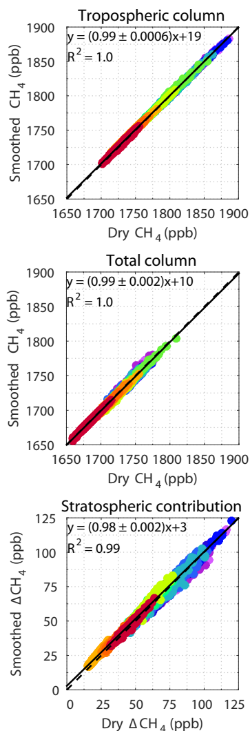
Figure B4. GEOS-Chem smoothed vs. dry integrated CH 4 DMFs for base simulation tropospheric columns, total columns, and stratospheric contribution. Site colors are as in Fig. 1. Dashed lines mark the one-to-one lines.
