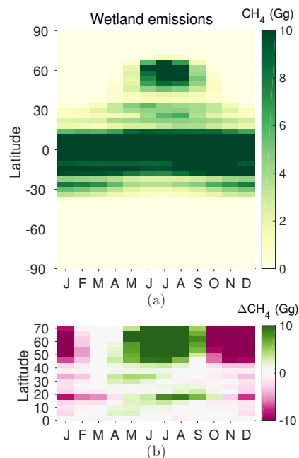
Figure 10. (a) GEOS-Chem monthly zonal mean wetland emissions, in Gg. (b) The Northern Hemisphere sensitivity of GEOS-Chem wetland emission attribution caused by a 3-month lag for each 1 ppb increase of \text{CH}_4 in the tropospheric column, in Gg.
