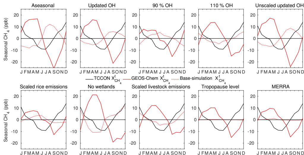
Figure B3. Seasonality of tropospheric methane ( X^t_{\text{CH}_4} ) at Park Falls for TCCON (black solid line), GEOS-Chem (red solid line), and the difference from the base simulation (dotted red line) for each of the sensitivity experiments, in ppb.
