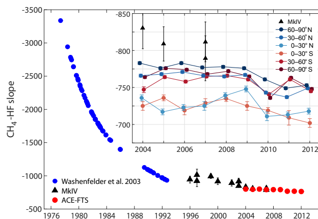
Figure A1. Long-term \text{CH}_4 -HF slopes from Washenfelder et al. (2003), MkIV, and updated ACE-FTS measurements. Inset: Time series of zonal pressure-weighted ACE-FTS slopes ( \beta ) used to calculate \hat{X}_{\text{CH}_4}^t , with error bars denoting the 2\sigma standard error. Zonal slopes are offset each year for visual clarity.
