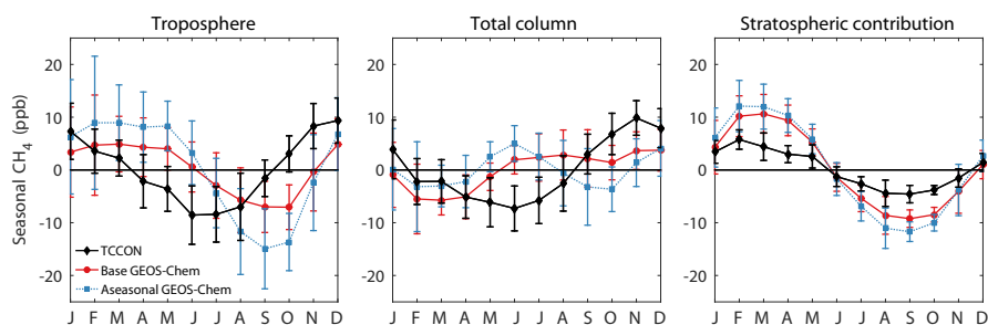
Figure 7. Detrended seasonality of TCCON (black diamonds), GEOS-Chem base (red circles), and GEOS-Chem aseasional (blue squares) \text{CH}_4 column-averaged DMFs, averaged across Northern Hemisphere sites, excluding Saga, which has less than one year of measurements prior to 2012. Error bars denote the 1\sigma standard deviation across sites.
