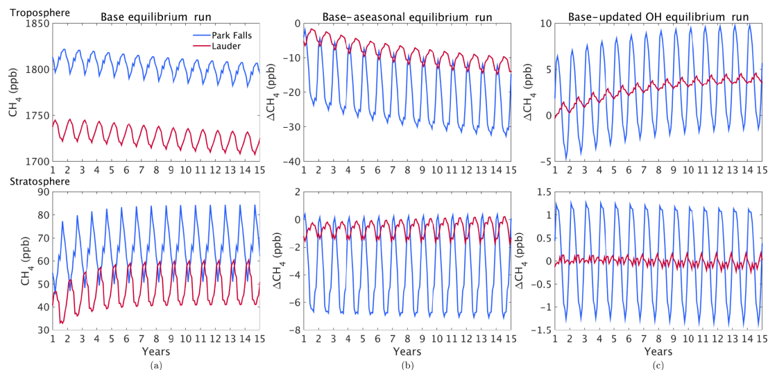
Figure 3. Smoothed daily mean X_{\text{CH}_4}^{\text{l}} and stratospheric contribution to X_{\text{CH}_4} at Park Falls (blue) and Lauder (red) for (a) base equilibrium simulation and the difference between the base and (b) aseasonal and (c) updated OH simulations.
