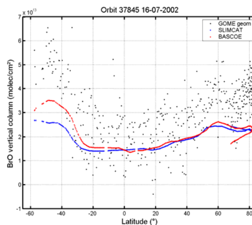
Fig. 7. BrO vertical columns derived from BASCOE and SLIMCAT models for a GOME orbit on 16 July 2002. GOME data are also displayed for comparison.
