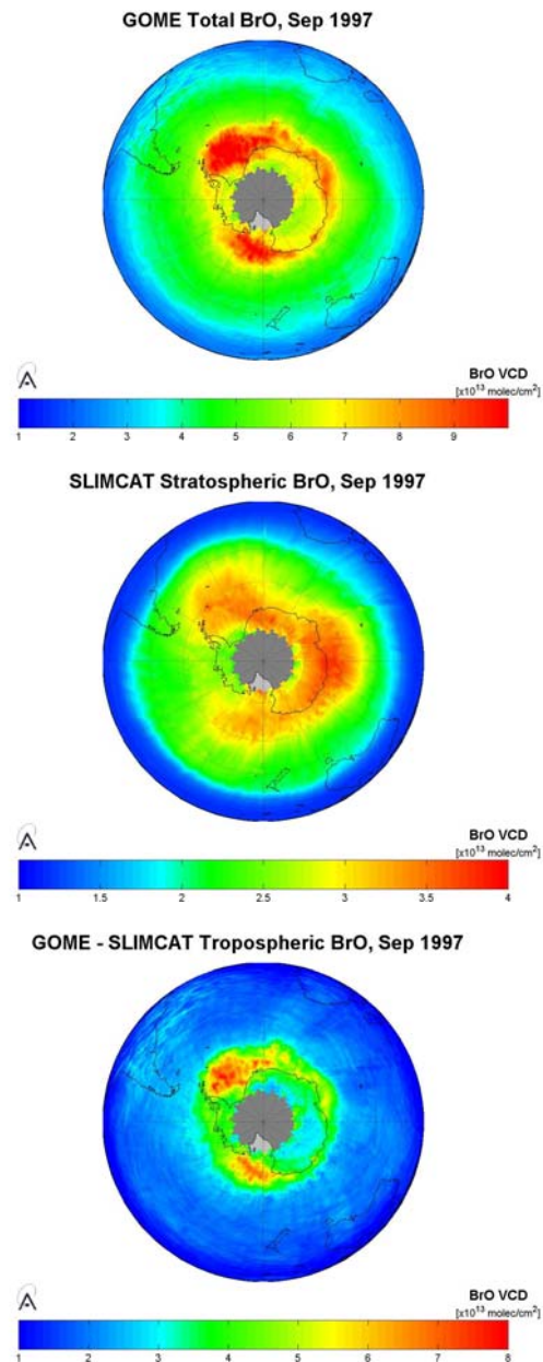
Fig. 5. BrO products for September 1997 in the southern hemisphere. (up) total VCD, (middle) stratospheric VCD, (bottom) tropospheric VCD.
