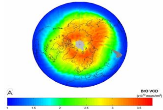
Fig. 2. SLIMCAT stratospheric BrO distribution for March 2001.
