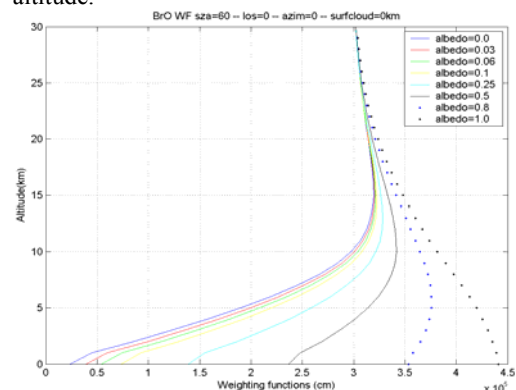
Fig.3. BrO weighting functions for different ground albedo. Calculations are for a solar zenith angle of 60° in a pure nadir viewing geometry.
