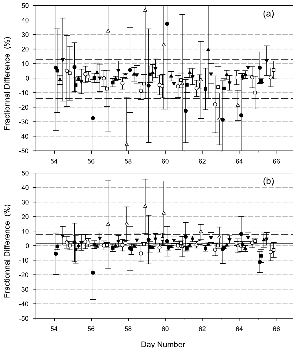
Figure 8. Daily (a) am and (b) pm averages of the fractional differences for all groups and TC1 settings. The error bars represent the standard deviation (solid circles, CNRS; solid squares, IASB_1; solid triangles, INTA; solid inverted triangles, IUPB_2; solid diamonds, IUPH; open circles, NILU_2; open squares, NIWA_2; open triangles, ULEI).
