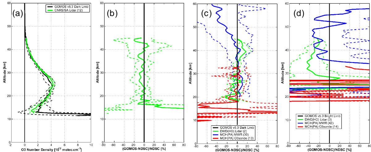
Fig. 3. Comparison between GOMOS and NDSC ozone profiles in the Alps. (a) Mean (continuous line) and standard deviation (dashed line) of 12 number density profiles measured at OHP by GOMOS in dark limb and by the CNRS lidar. (b) Percent relative difference and its standard deviation between the same GOMOS and lidar profiles as in (a). (c) Same GOMOS/NDSC differences as in (b), but at Hohenpeißenberg with DWD lidar and at Payerne with MCH ozonesonde and MWR. (d) Same GOMOS/NDSC differences as in (c), but using GOMOS bright limb data.
