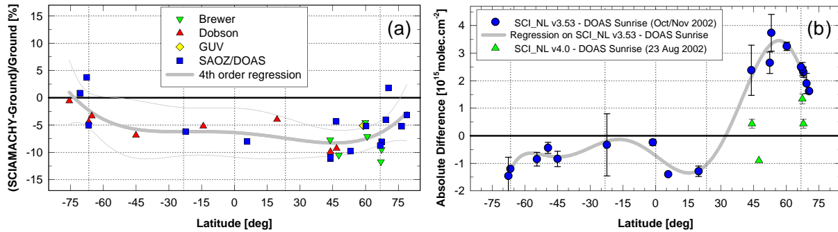
Fig. 1. Mean difference between early SCIAMACHY and ground-based column measurements as a function of the latitude. (a) Percent relative difference between Meteo v3.53 and ground-based total ozone: A general underestimation of ground-based values by SCIAMACHY vanishes near the poles. (b) Absolute difference between NRT v3.53 and ground-based total nitrogen dioxide: A strong meridional structure appears, that might be related to the use of an improper atmospheric profile database for the calculation of the SCIAMACHY AMF. Preliminary v4.0 results suggest some possible improvement.
