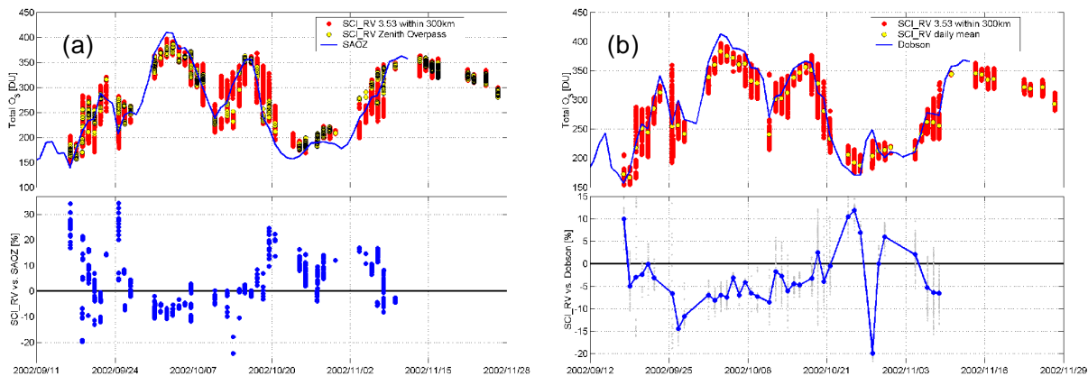
Fig. 2. Comparison of SCIAMACHY v3.53 with ground-based total ozone at two neighbouring NDSC/Antarctic stations: (a) with BAS SAOZ data at Rothera (68°S), and (b) with the KTSU/BAS Dobson data at Vernadsky (65°S). Upper panels: time-series of total ozone observed by SCIAMACHY (two methods of selection) and the ground-based instrument; lower panels: time-series of relative differences. Although the average agreement is excellent, systematic differences of \pm 15\% are frequent. Those differences correlate with the ozone column value. The reduction of the scatter gained by a physically based selection method is well illustrated by the SCIAMACHY/SAOZ comparisons in (a).
