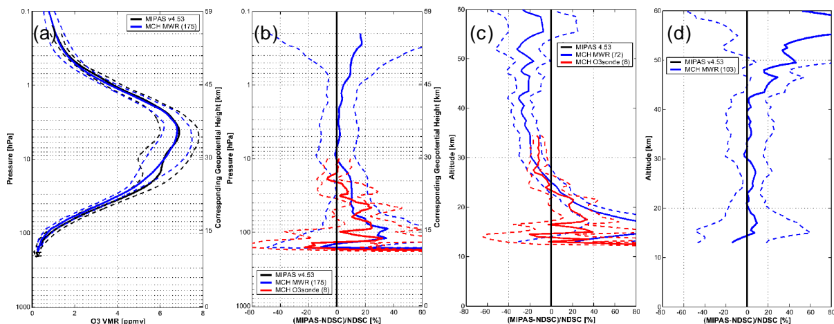
Fig. 4. Comparison between MIPAS and correlative ozone profiles at the NDSC/Alpine station of Payerne. (a) Mean (continuous line) and standard deviation (dashed line) of 175 VMR profiles in log-pressure scale, measured by MIPAS and by the millimetre wave radiometer (MWR). (b) Percentage relative difference between MIPAS and ground-based (MWR and ozonesonde) ozone VMR. (c) Same as (b), but on an altitude grid and with 72 MIPAS profiles acquired before November 13, 2002 12 h UT. (d) Same as (c), but with 103 MIPAS profiles after November 13, 2002 12 h UT.
