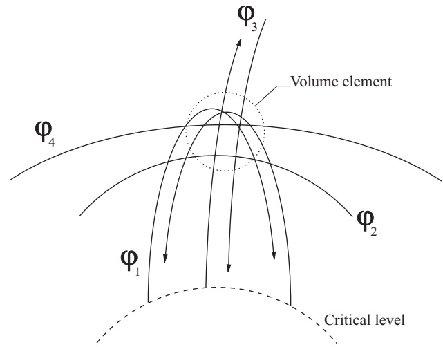
Fig. 13. Exospheric particles.
