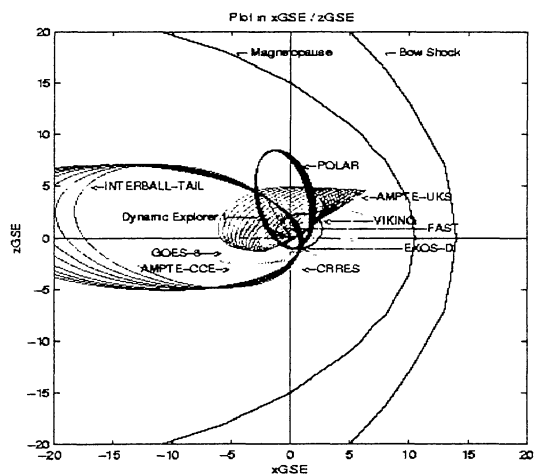
Figure 5: Projection in the (X_{GSE}, Z_{GSE}) plane of the first twenty orbits of ten satellites listed in this catalogue.
