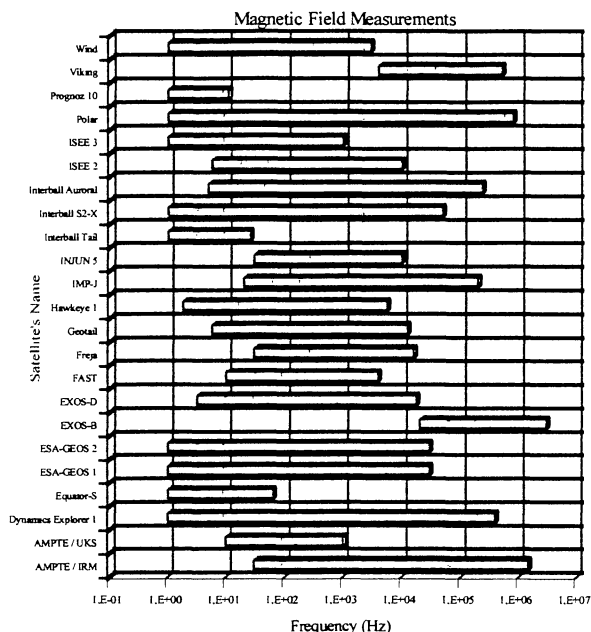
Figure 4: Frequency ranges for which magnetic field observations have been collected for some satellites of the database.
