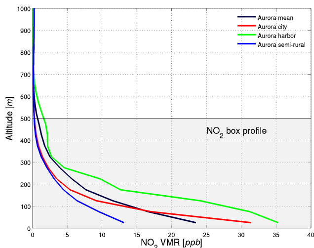
Figure 11. Representative AURORA a priori NO 2 profiles used for the Antwerp data set RTM calculations. A simple NO 2 box profile of 500 m height which is well-mixed in the boundary layer is also used in the sensitivity study.
