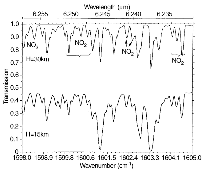
Fig. 6. Simulated atmospheric spectra in the 1598\text{--}1605\text{ cm}^{-1} spectral range containing significant \text{NO}_2 absorptions, corresponding to MIRAS measurements at different tangent altitudes ( H = 15, 30\text{ km} )
