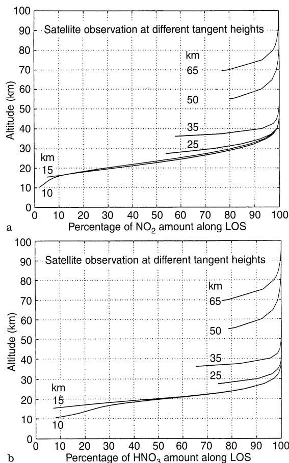
Fig. 4a, b. Growth of the accumulated molecular amount along the line-of-sight (LOS) versus altitude above earth's surface, for a satellite limb observation (from MIRAS) at different tangent heights (TGP) of a NO 2 , b HNO 3
