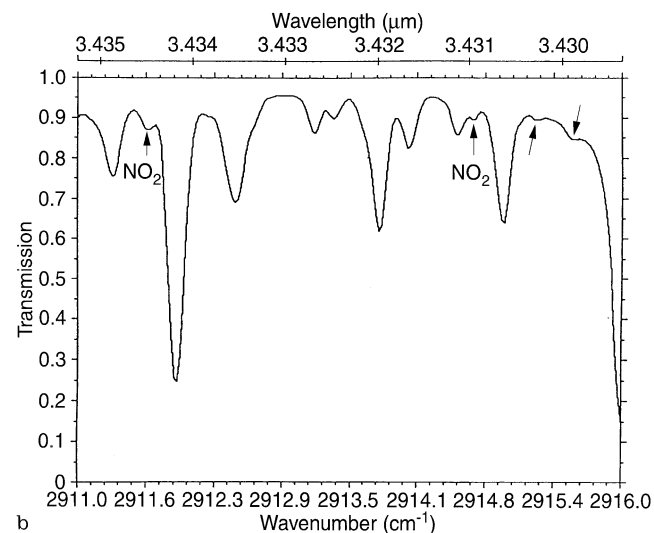
Fig. 8a, b. Simulated ground-based atmospheric spectrum in the 2911\text{--}2916\text{ cm}^{-1} spectral range, containing characteristic \text{NO}_2 absorptions, a at solar zenith angle (SZA) = 26^\circ , b at SZA = 76^\circ
