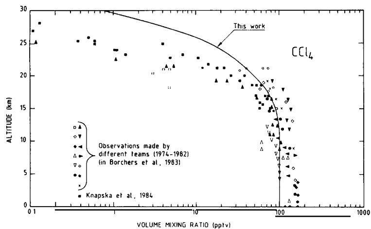
Fig. 5. Comparison between observed distributions of carbon tetrachloride [8, 9] and a 1-D theoretical profile.
