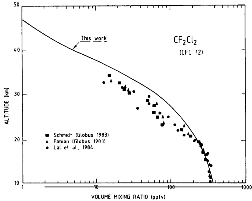
Fig. 4. Comparison between observed distributions of CFC-12 [3, 5] and a 1-D theoretical profile.
