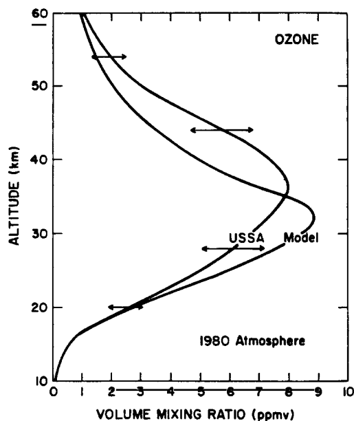
Fig. 12. Comparison between the U.S. Standard atmosphere model of ozone [21] and a theoretical vertical distribution.
