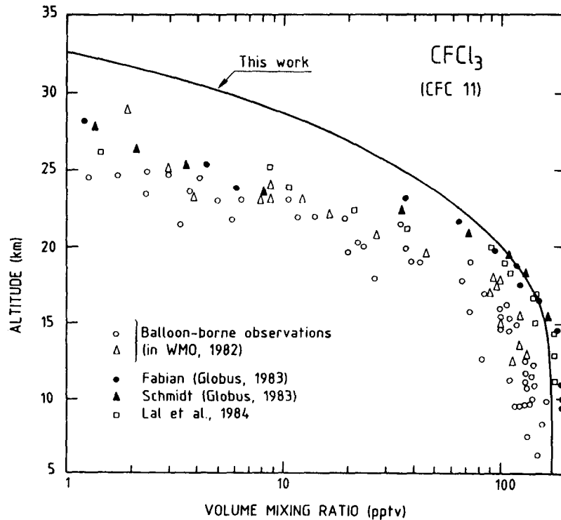
Fig. 3. Comparison between observed distributions of CFC-11 [3, 5] and a 1-D theoretical profile.
