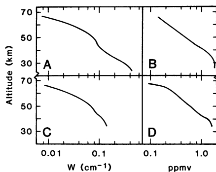
Fig. 2. (A) Equivalent width, W , of the absorption feature at 3017.8\text{ cm}^{-1} as a function of tangent altitude of the line of sight to the sun center. (B) Inverted \text{CH}_4 volume mixing ratio computed on the basis of the U.S. standard atmosphere (1966) for the atmospheric temperature and total number density profile versus altitude. (C) Equivalent width of the 2979\text{-cm}^{-1} \text{CH}_4 manifold versus tangent altitude. (D) Deduced \text{CH}_4 vertical distribution (ppmv, parts per million by volume).
