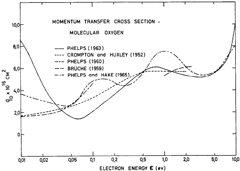
FIG. 2. ENERGY DEPENDENT MOMENTUM TRANSFER CROSS SECTION FOR ELECTRONS IN MOLECULAR OXYGEN.
