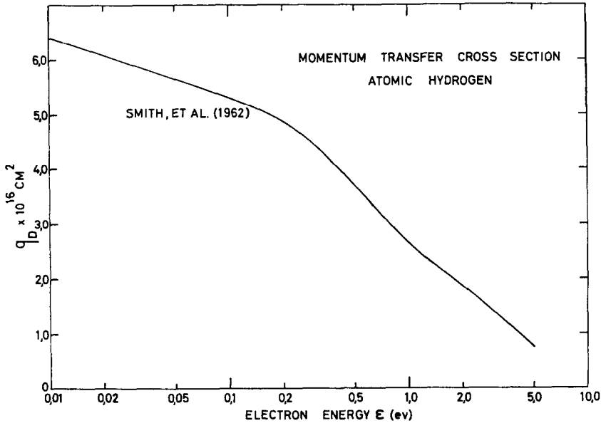
FIG. 4. ENERGY DEPENDENT MOMENTUM TRANSFER CROSS SECTION FOR ELECTRONS IN ATOMIC HYDROGEN.
