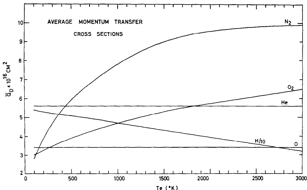
FIG. 5. AVERAGE MOMENTUM TRANSFER CROSS SECTIONS FOR ELECTRONS.
