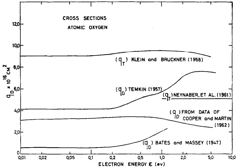
FIG. 3. ENERGY DEPENDENT CROSS SECTIONS FOR ELECTRONS IN ATOMIC OXYGEN. The data of Klein and Brueckner (28) and Neynaber et al. (28) apply to the total scattering cross section. The phase shift data of Cooper and Martin (26) are used here to calculate values of q_D . The data of Temkin (27) and Bates and Massey (28) originally included only S -wave phase shifts. These have been expanded for the purposes of comparison using the P -wave shifts of Cooper and Martin. (26)
