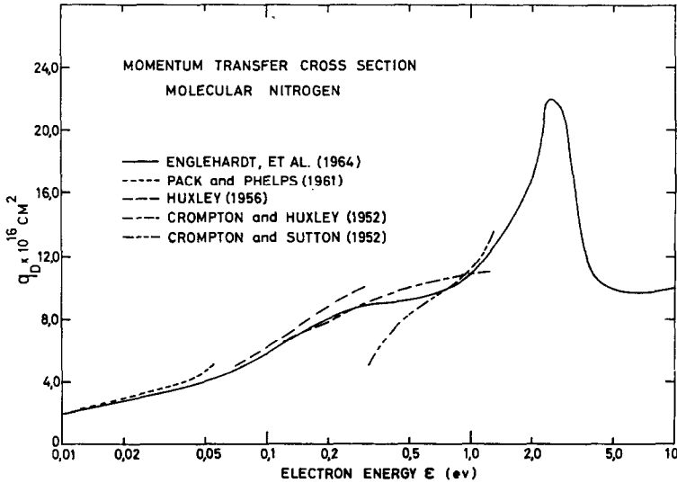
FIG. 1. ENERGY DEPENDENT MOMENTUM TRANSFER CROSS SECTION FOR ELECTRONS IN MOLECULAR NITROGEN.
