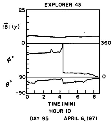
Fig. 1. Example of a discontinuity. In this case the direction of the magnetic field changed by 75^\circ , somewhat larger than the average ( 60^\circ ). This satisfies the definition for a directional discontinuity introduced by Burlaga [1969].
