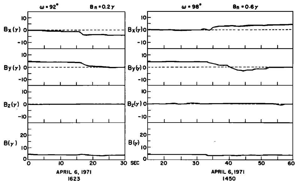
Fig. 11. Structure of two TD's. In both cases the magnetic field intensity is nearly constant, and the field vector rotates in a plane. The component normal to this plane ( B_z ) is consistent with zero in both cases, indicating that the discontinuities are tangential.
