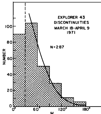
Fig. 3. Distribution of \omega , the change in direction of the magnetic field, across the discontinuities that were selected. For 31% of the discontinuities, \omega < 30^\circ . The curve for \omega > 30^\circ is N = N_0 \exp(-\omega/75^\circ) , which is the same function that Burlaga [1969] found for the \omega distribution of directional discontinuities in Pioneer 6 data.
