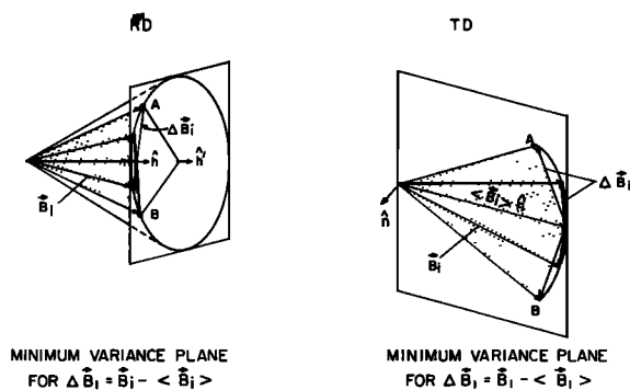
Fig. 6. For an RD (left) the magnetic field rotates on the surface of a cone, while for a TD (right) it rotates in a plane. The Sonnerup-Cahill method determines the plane which contains \Delta \mathbf{B}_i = \mathbf{B}_i - \langle \mathbf{B}_i \rangle . For an RD there is a nonzero component of B normal to this plane, while for a TD there is no component of B normal to this plane. The determination of the plane containing \Delta \mathbf{B}_i is uncertain when \omega is small because some of the \Delta \mathbf{B}_i are too small to measure accurately in this case.
