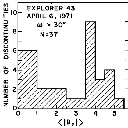
Fig. 13. Distribution of \langle |B_z| \rangle for the discontinuities on April 6. It is bimodal and suggests equal numbers of TD's and RD's.
