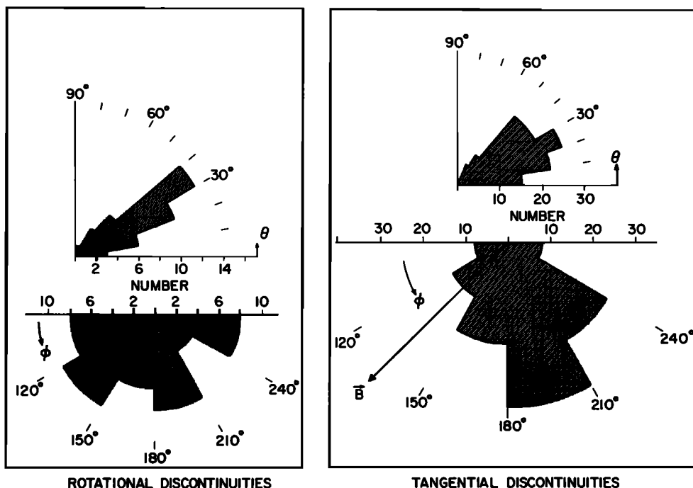
Fig. 9. Distribution of the normals to the surfaces of TD's and RD's. Both tend to be above the ecliptic plane. The TD normals tend to be normal to the spiral field, whereas the RD normals are more isotropically distributed.
