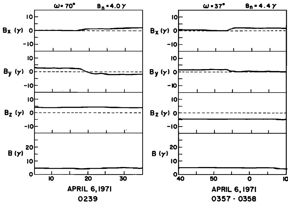
Fig. 12. Structure of two RD's. The magnetic field intensity is constant, and the magnetic field rotates on a cone. The component B normal to the base of the cone is large in both cases, indicating that the discontinuities are rotational.
