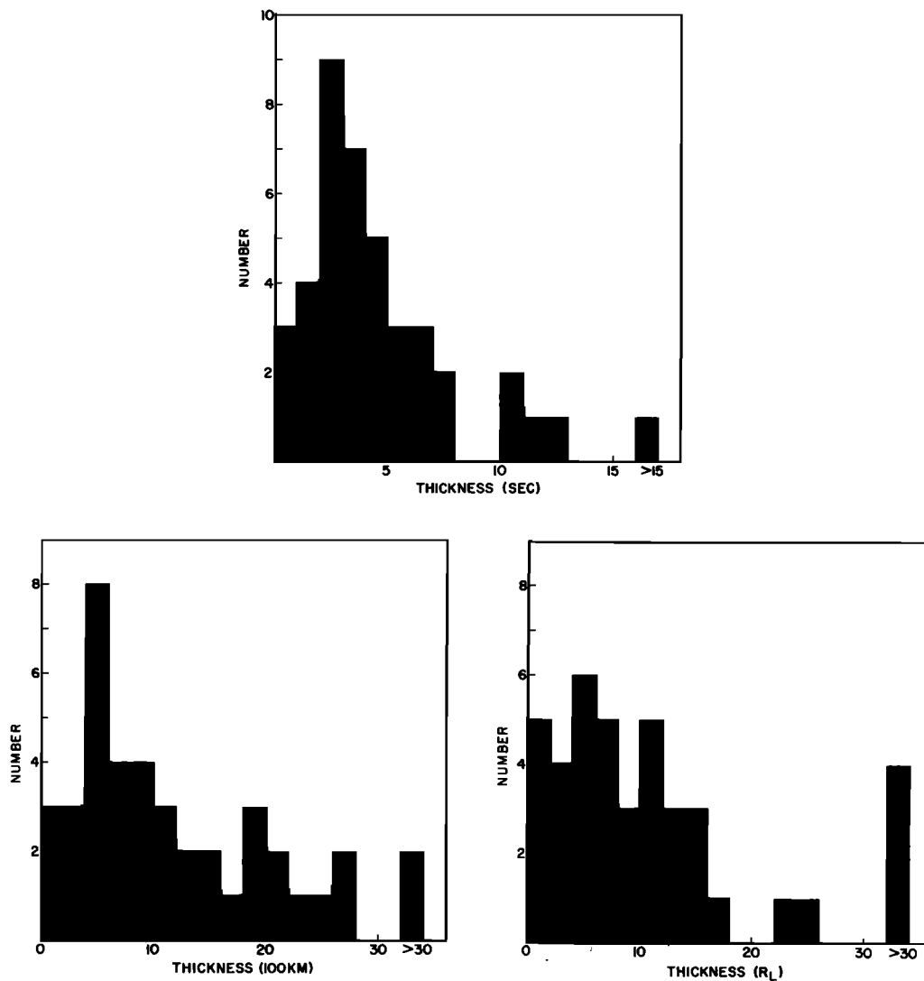
Fig. 14. Thickness distributions for TD's.
