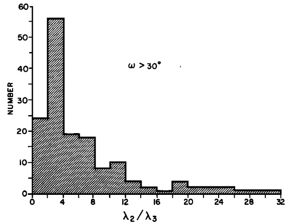
Fig. 7. Distribution of the ratio of the intermediate eigenvalue \lambda_2 to the minimum eigenvalue \lambda_3 from the minimum variance analysis of the \Delta \mathbf{B}_i . This quantity must be large if one is to determine accurately the minimum variance plane of \Delta \mathbf{B}_i . One sees that it is large for most of the discontinuities with \omega > 30^\circ .
