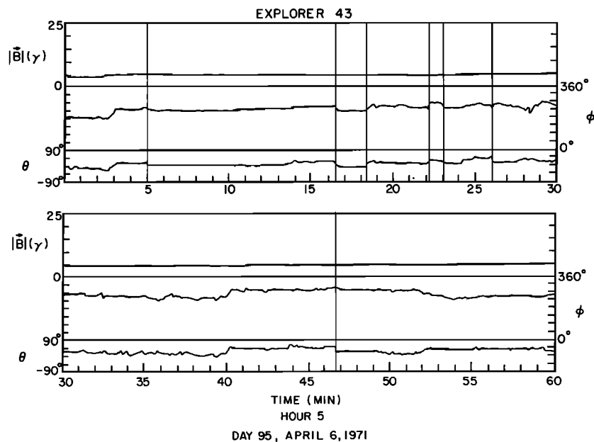
Fig. 2. Examples of other discontinuities that were selected. The events shown here do not satisfy the definition of a directional discontinuity because the change in direction \omega is small and/or the discontinuities are too close together. They were included in the initial selection because the changes appear to be nearly discontinuous.
