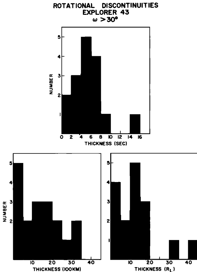
Fig. 15. Thickness distributions for RD's.
