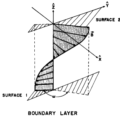
Fig. 5. The transition between the two sides of a 'discontinuity' is actually a continuous one and is called a boundary layer or current sheet. For a TD the magnetic field vector rotates in the boundary layer from one state to another, always remaining parallel to the surface of the 'discontinuity,' as shown here. For an RD, one component of B rotates as shown here, and in addition, there is a component of B perpendicular to the surface of the 'discontinuity.'
