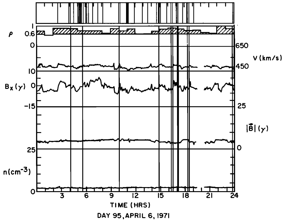
Fig. 10. An Alfvénic period. The fluctuations in V and B_x are highly correlated (the correlation coefficient \rho being greater than 0.6 throughout the day), and the density and magnetic field intensity are relatively constant, indicating Alfvénic fluctuations. Forty-five discontinuities were observed during this day, shown by the vertical lines in the top panel. Several of these were tangential discontinuities, indicated by the vertical lines extending through all of the panels.
