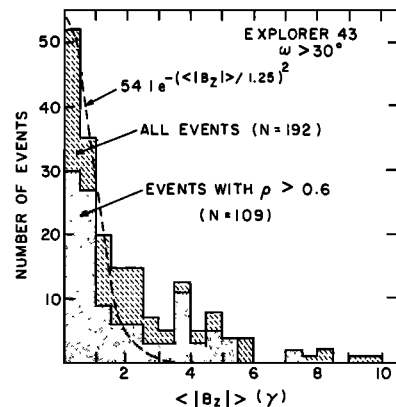
Fig. 8. Distribution of \langle |B_z| \rangle , the component of B normal to the minimum variance plane of \Delta \mathbf{B}_i . Only discontinuities with \omega > 30^\circ are considered, so that the minimum variance plane is well determined. The peak is at \langle |B_z| \rangle = 0 , and there is a population of events with \langle |B_z| \rangle < 2 \gamma , consistent with TD's. There is another population with \langle |B_z| \rangle > 3 \gamma , consistent with RD's. The ratio of TD's to RD's obtained in this way is 2.8 to 1. One obtains essentially the same distribution when only Alfvénic ( \rho > 0.6 ) periods are considered.
