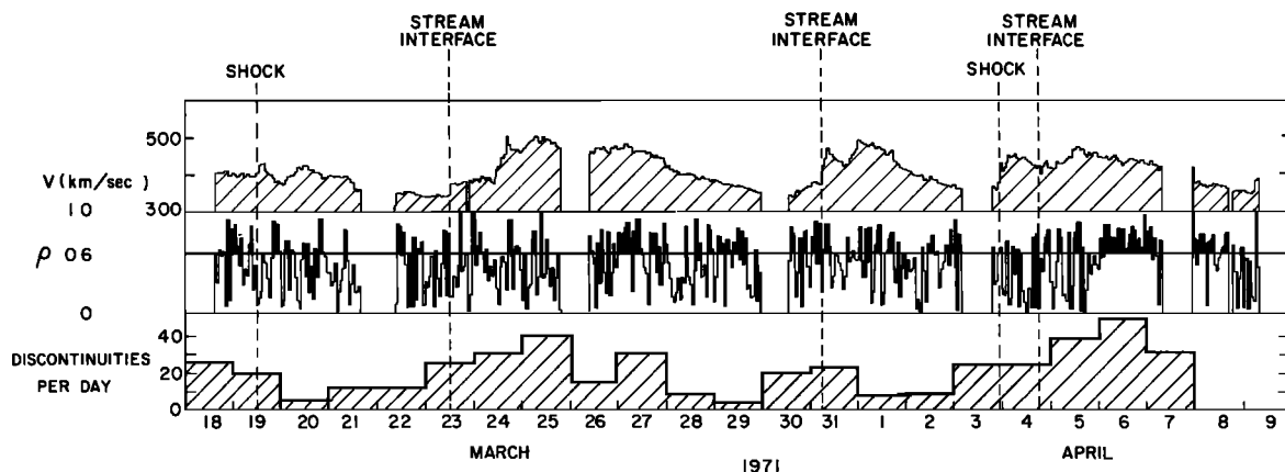
Fig. 4. (Top) Flow configuration in the period that is considered in this paper, (middle) correlation \rho between speed and the radial component of the magnetic field, which indicates the presence of Alfvénic fluctuations when it is large ( > 0.6 ), and (bottom) number of discontinuities per day as a function of time. The main point is that the discontinuities that we selected are found under a wide variety of interplanetary conditions.
