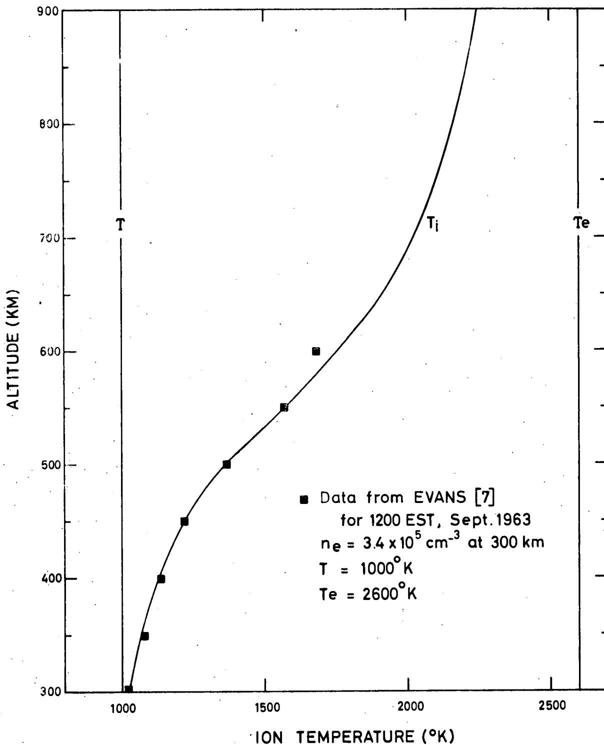
Fig. 4.- Comparison of calculated and measured ion temperatures. The solid curve was calculated using a 1000^\circ \text{K} model neutral atmosphere and the experimental parameters of Evans [7]. The squares indicate the measured values.
