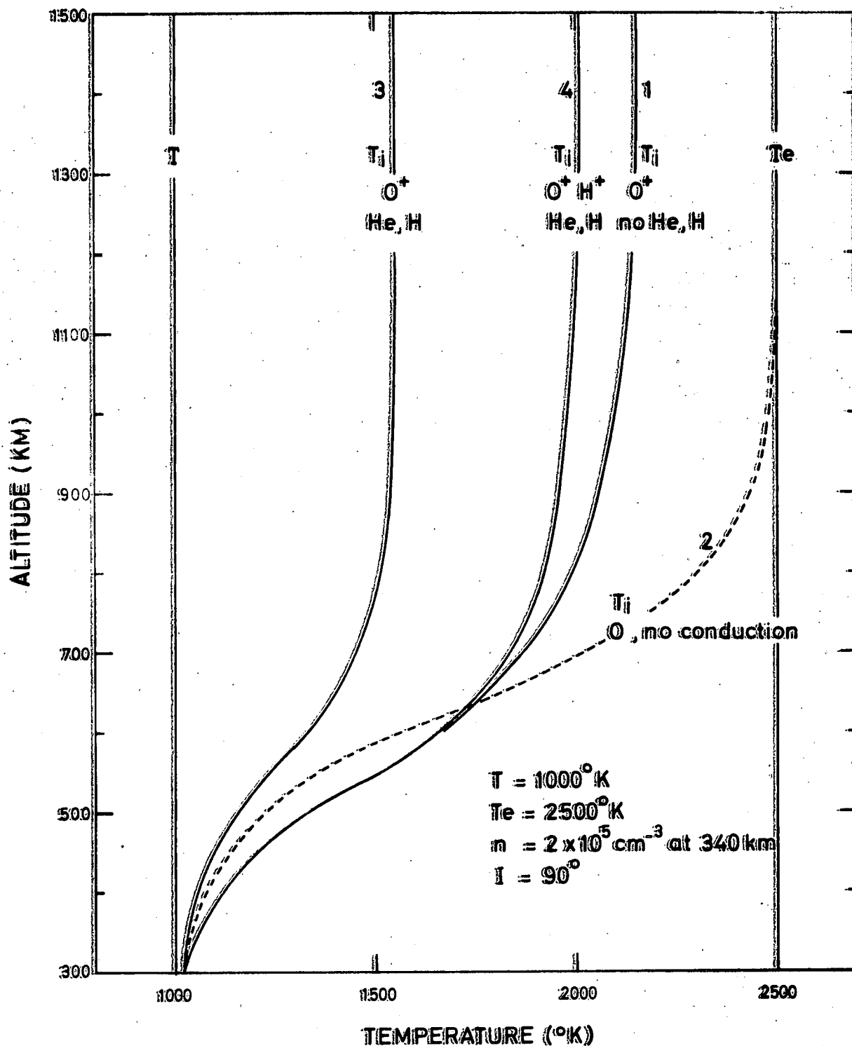
Fig. 1.- Ion temperatures with an electron temperature of 2500^{\circ} K and neutral gas temperature of 1000^{\circ} K, for a magnetic dip angle of 90^{\circ} with an electron density of 2 \times 10^5 \text{ cm}^{-3} at 340 km. Curve 1 includes O^+ ions and thermal conduction but neglects cooling by He and H. In curve 2 the same conditions are used with no thermal conduction. Curve 3 includes O^+ ions, thermal conduction, He and H. Curve 4 represents the final result with O^+ , H^+ , He, H and thermal conduction.
