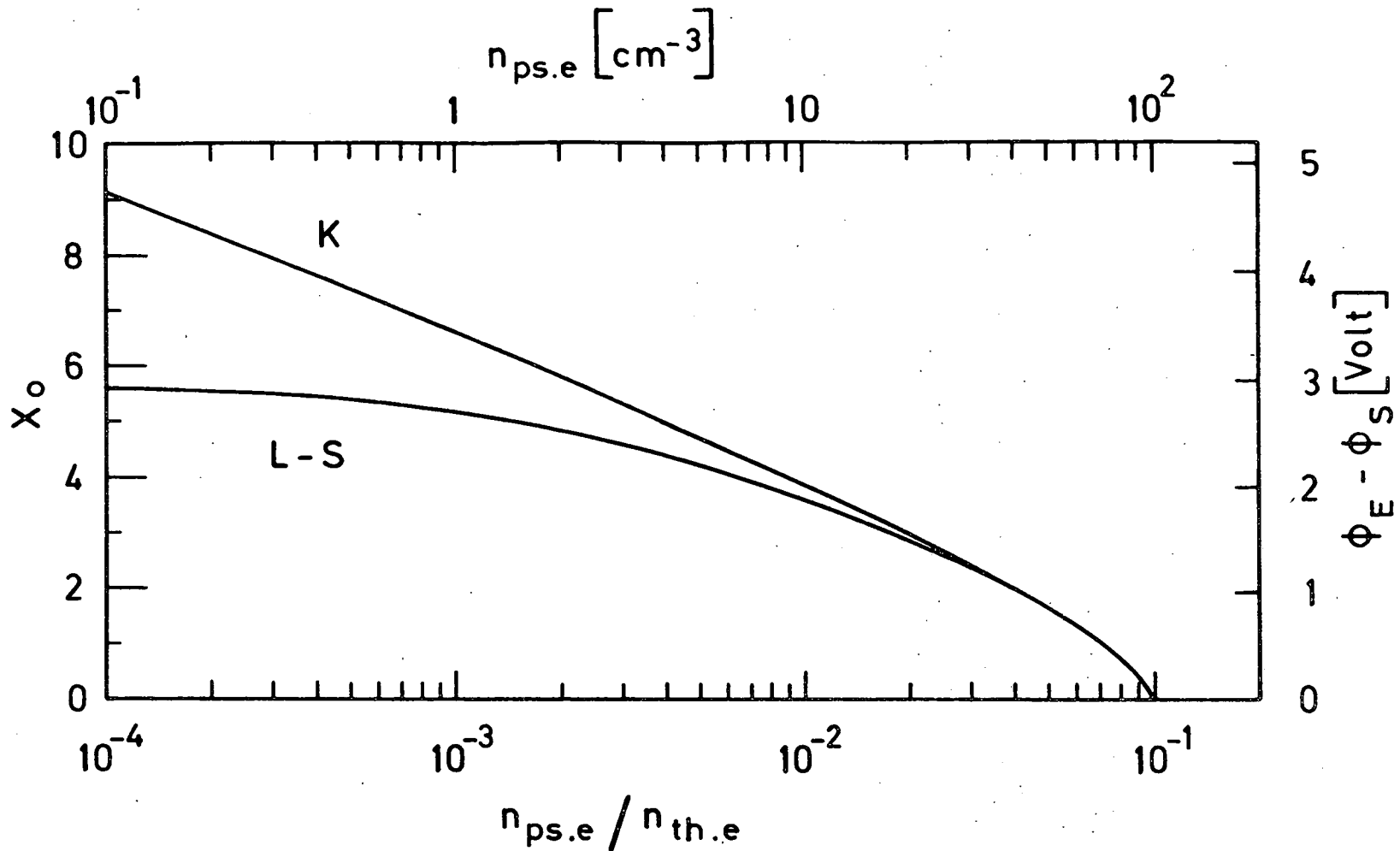
Fig. 2.- Electric potential difference between the ionosphere ( E ) and the plasmashet ( S ) required to balance the upward and downward currents carried by the hot plasmashet and cold ionospheric particles (i.e. \Sigma j = 0 ). As for Fig. 1 it is assumed that n_{th,e} = 10^3 \text{ cm}^{-3} , T_{th,e} = 6000 \text{ }^\circ\text{K} , T_{ps,e}/T_{th,e} = 10^2 , A_S/A_E = B_E/B_S = 10^3 . The density of the precipitating plasmashet electrons is varied from n_{ps,e} = 10^{-1} \text{ cm}^{-3} to 10^2 \text{ cm}^{-3} . In Knight's (1973) model (K) where the current transported by the H^+ ions is neglected, the potential difference for a zero electric current increases indefinitely when n_{ps,e} tends to zero, while in Lemaire and Scherer's [1973] model (L-S) it has a maximum value: |\Phi_E - \Phi_S|^{max} = 2.92 \text{ Volt} . For n_{ps,e} > 10^2 \text{ cm}^{-3} , the potential difference for a zero electric current becomes negative and the flux of precipitating electrons is larger than the threshold for formation of double layers [Block, 1971] or for driving the ion-cyclotron waves unstable [Kindel and Kennel, 1971].
