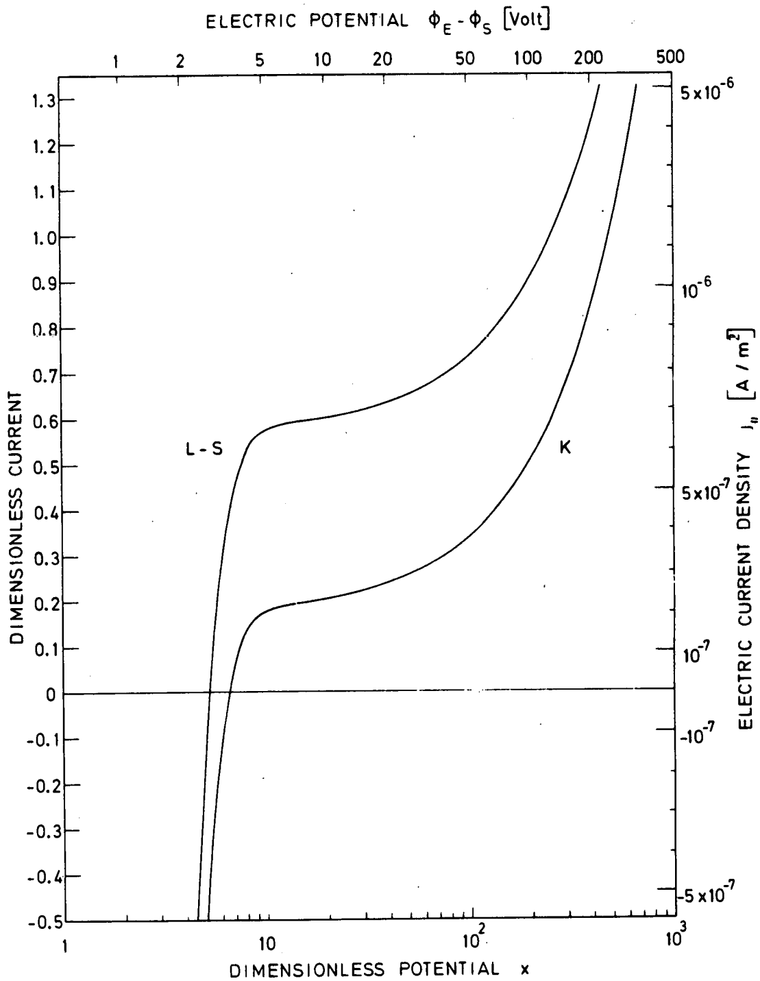
Fig. 1.- Parallel electric current density as a function of the electric potential difference between the ionosphere ( E ) and the plasmashet ( S ). The density and temperature of the thermal electrons at the ion-exobase are respectively: n_{th,e} = 10^3 \text{ cm}^{-3} , and T_{th,e} = 6000 \text{ }^\circ\text{K} . The density and temperature of the plasmashet electrons at the equatorial end of the magnetic line of force are respectively given by n_{ps,e} = 10^{-3} n_{th,e} , and T_{ps,e} = 10^2 T_{th,e} . It was also assumed that the equatorial cross section, A_S , of the auroral flux tubes is 1000 times larger than A_E , its cross-section in the ionosphere: A_S/A_E = B_E/B_S = 10^3 . The field-aligned current is zero for a potential difference of 3.39 Volts in Knight's [1973] model (K), and for \phi_E - \phi_S = 2.69 Volt in Lemaire and Scherer's [1973] model (L-S). Note the non-linearity of the Electrical Characteristics of the collisionless plasma distributed along an auroral field line.
