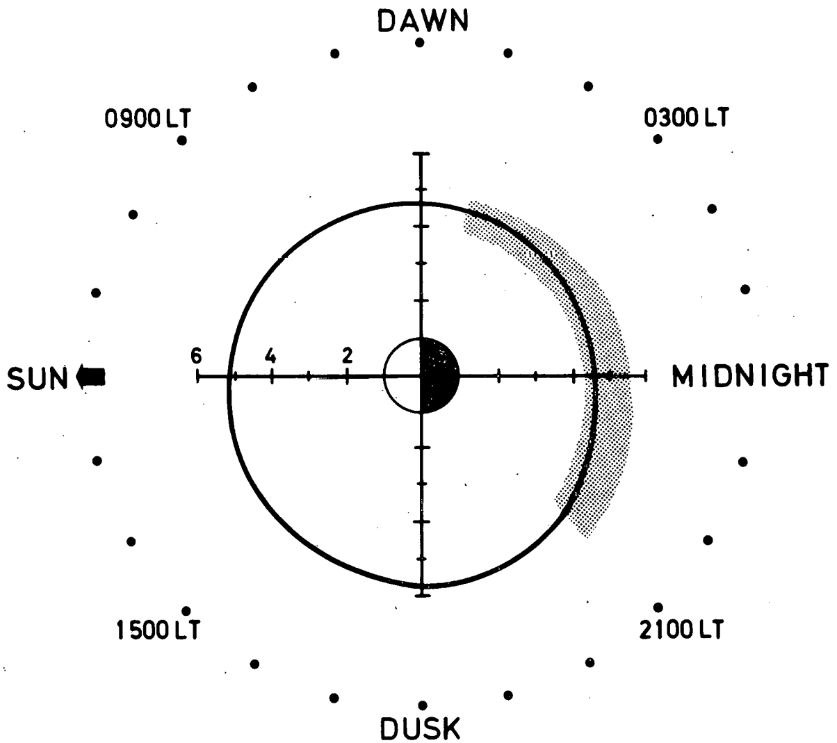
Fig. 13.- Local time variation of the plasmopause ; the solid line is the steady state plasmopause equatorial section deduced from the E3H model of McIlwain [1974], for K_p = 1-2 . The shaded area corresponds to the region where the night time plasmopause is to be found when K_p = 1 according to the Rycroft and Burnell [1970] statistical analysis of Carpenter's [1966] whistler observations.
