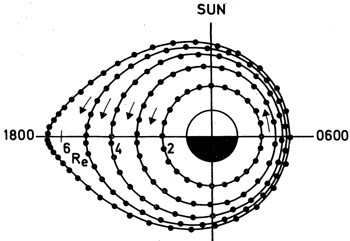
Fig. 4.- Drift paths of cold plasma elements inside of a 'tear-drop' model of the plasmasphere; the dots represent the successive positions of whistler ducts, separated by 1 hour intervals of time. The angular drift velocity is expected to be larger (smaller) than the rotation speed of the Earth, in the dawn (dusk) region.
