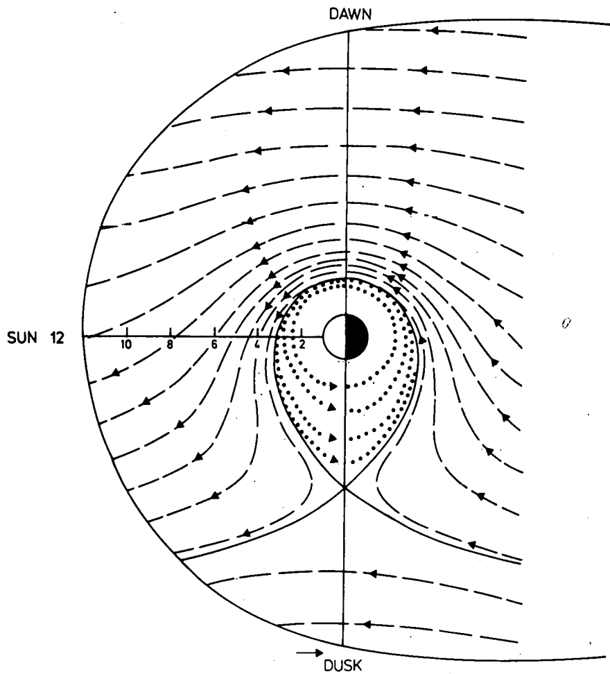
Fig. 3.- The 'tear-drop' model of the plasmasphere; equipotentials of the combined corotation and uniform dawn-dusk electric fields. [Kavanagh, et al. , 1968]. The plasmasphere has a 'tear-drop' shape. The position of the stagnation point at 1800 LT depends on E_0 , the intensity of the uniform dawn-dusk field; E_0 = 0.3 mV/m in the illustrated case.
