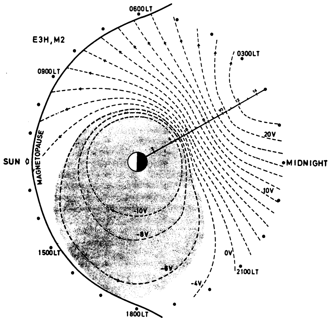
Fig. 8. Magnetospheric electric field model E3H of McIlwain [1974] ; the dashed curves represent the equatorial sections of equipotential surfaces. The last 'closed' equipotential corresponds to the outer boundary of the light shaded area which represents the plasmasphere according to the MHD theory of the formation of the plasmapause.
