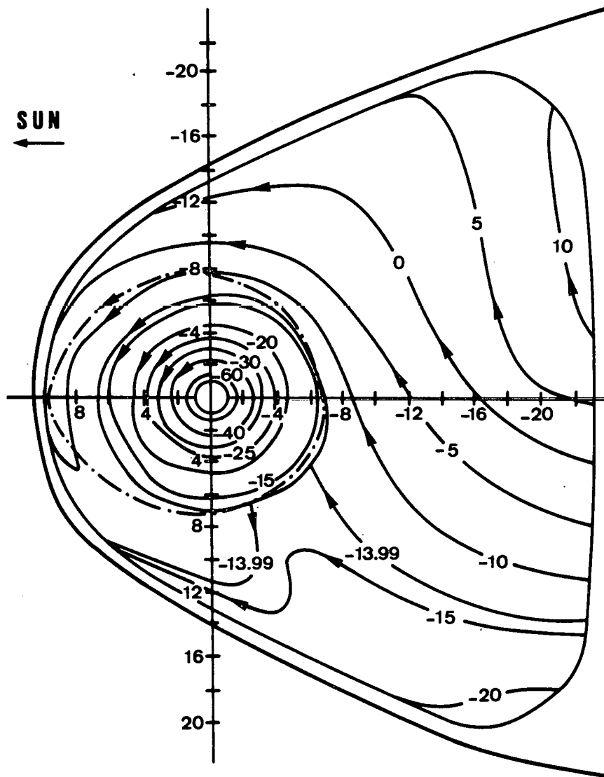
Fig. 6.- Magnetospheric electric field model including ionospheric conductivities and a thin ion-sheet in the equatorial plane; energetic ions are injected with 90^\circ pitch angles into the equatorial plane of the magnetosphere; the resulting equipotential surfaces differ significantly from those obtained without this ion-sheet [Wolf, 1974].
