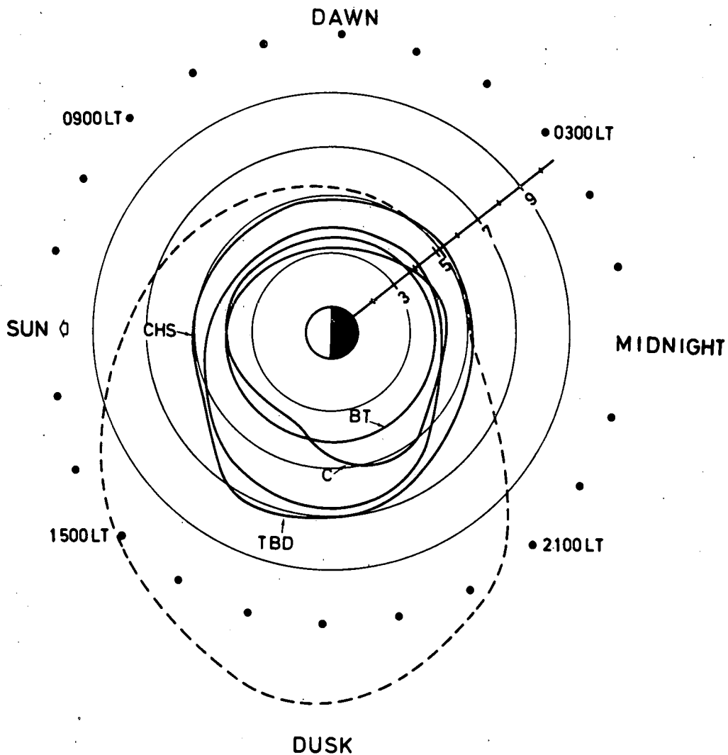
Fig. 9.- Observed positions of the plasmopause ; (C): from whistler observations, for steady geomagnetic agitation ( K_p = 2-4 ) [Carpenter, 1966]; (CHS): average plasmopause position determined from more than 150 OGO 5 thermal ion density profiles [Chappell et al. , 1971]; (TBD): plasmopause positions from OGO 3 ion spectrometer measurements for K_p = 2-4 [Taylor et al. , 1970]; (BT): from ISIS 1 electrostatic probe measurements, for K_p < 4 [Brace and Theis, 1974]. The dashed curve is the last 'closed' equipotential in the E3H model of McIlwain [1974].
