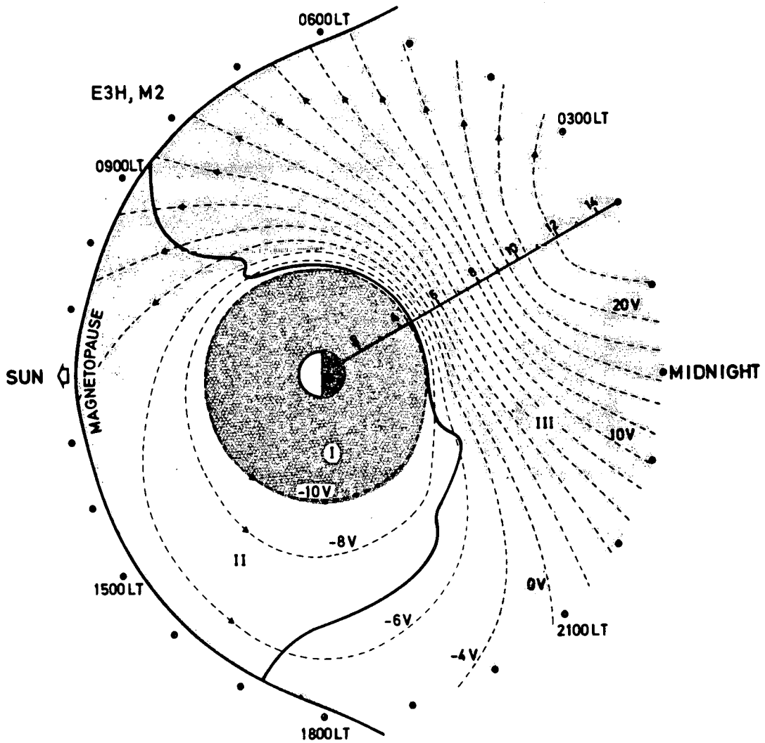
Fig. 12.- The 'Roche Limit' surface for the E3H model of McIlwain [1974]; the dashed lines are electrostatic equipotentials. The solid line is the equatorial section of the 'Roche Limit' surface where the total potential, \phi_t , has a maximum. The boundary of the inner shaded region I is tangent to the 'Roche Limit' surface near midnight; the inner boundary of the outer shaded region III is the last 'closed' electric equipotential surface.
