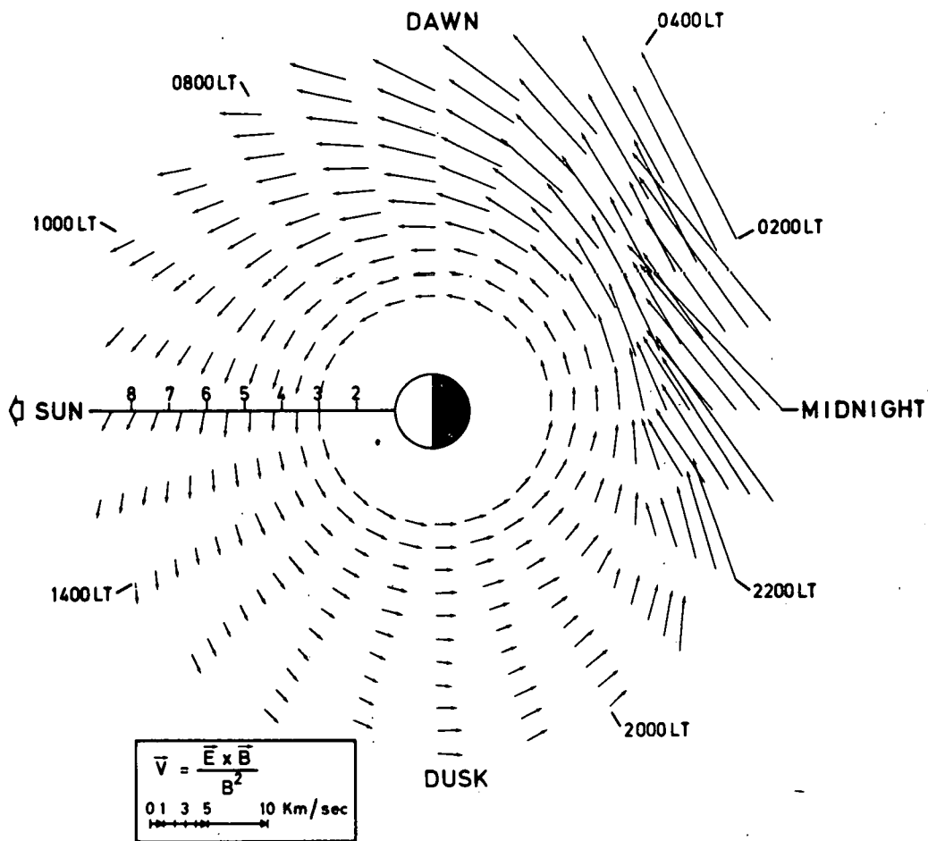
Fig. 11.- Electric drift velocities associated with the electric and magnetic field models E3H and M2 of McIlwain [1974]; for L < 4.5 the drift speed is nearly equal to the corotation velocity. A large increase of the eastward drift speed is seen in the midnight sector beyond L = 4.5 .
