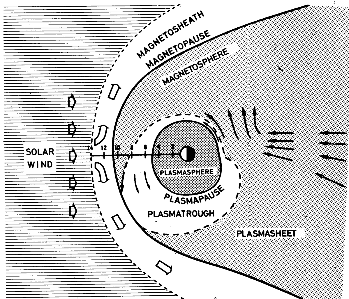
Fig. 14.- Equatorial section of the magnetospheric regions; summary diagram.
