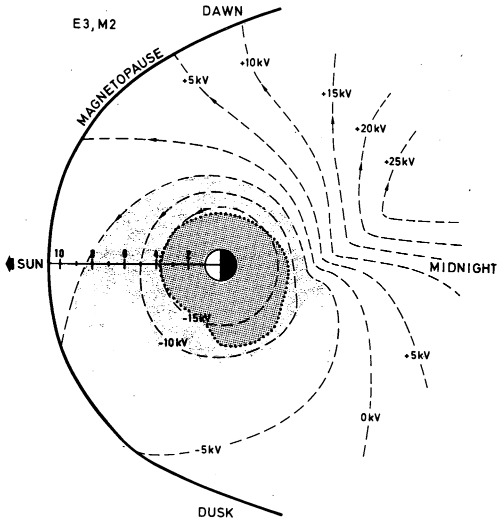
Fig. 7.- Magnetospheric electric field model E3 of McIlwain [1972] ; the dashed curves represent the equatorial sections of equipotential surfaces. The last 'closed' equipotential corresponds to the outer boundary of the light shaded area which represents the plasmasphere according to the MHD theory of the plasmapause formation. The positions of the plasmapause observed by Carpenter [1966] are shown by dots.
