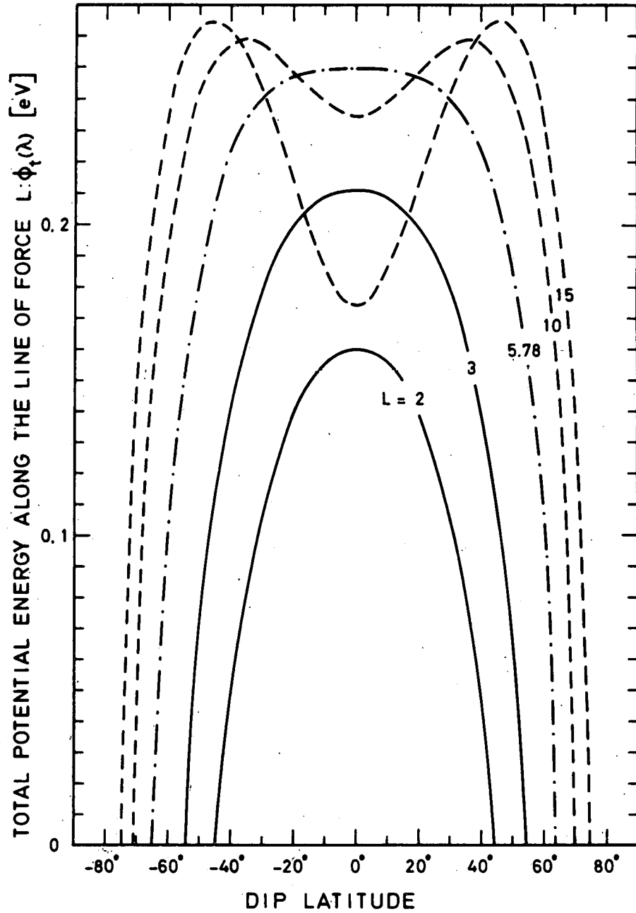
Fig. 10.- Gravitation plus rotation potential energy of an H^+ ion along different dipole magnetic field lines corotating with the Earth; for L \leq 5.78 , the total potential, \phi_t , has a maximum in the equatorial plane; for L > 5.78 , \phi_t has a minimum at the equator and two symmetric maxima out of the equatorial plane.
