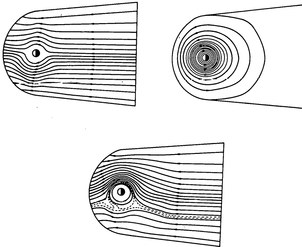
Fig. 2.- Magnetospheric electric field model proposed by Brice [1967]; Equatorial section of equipotential surfaces of the electric field induced into the magnetosphere by the solar wind (a), and by the corotation of the ionosphere (b). The combined field (c) is a 'best-estimate' determined to reproduce as closely as possible the plasmopause positions observed by Carpenter [1966].
