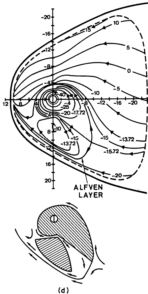
Fig. 5.- Magnetospheric electric field model taking into account finite transverse electric conductivities in the ionosphere; a 'best guess' non-uniform ionospheric conductivity is adopted with ad-hoc boundary conditions at the magnetopause to compute the equatorial section of the equipotential surfaces. The shaded areas are enveloped by the last 'closed' equipotential surfaces, and correspond to the plasmasphere in the MHD approximation [Wolf, 1970].
