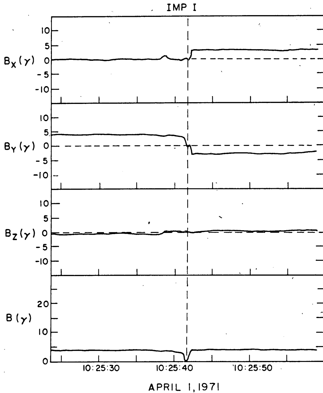
Fig. 4.- A magnetic hole which resembles a magnetic merging region but in which the minimum field intensity is lower than expected from the merging hypothesis.
