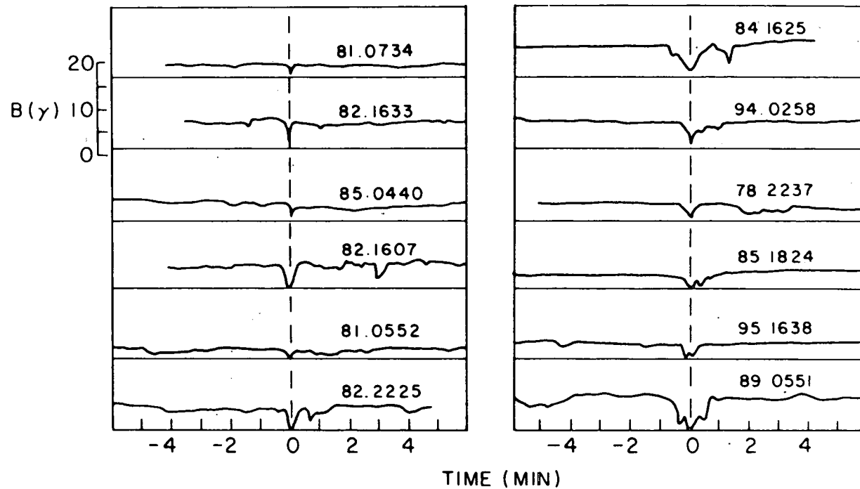
Fig. 1.- Representative examples of magnetic holes. In each panel, 15 s averages of the magnetic field intensity are plotted versus time. The events are labeled by decimal day and universal time. Despite the variety of shapes and widths, there is a common characteristic, viz., a distinct depression to |\vec{B}| < 1 \gamma in an otherwise normal magnetic field profile.
