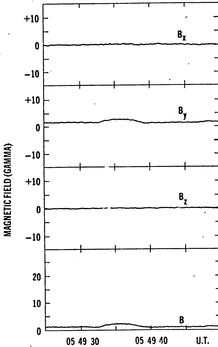
Fig. 6.- The antithesis of a magnetic hole. Here the magnetic field intensity increases in a 7 s. interval while the direction remains constant. Presumably the plasma pressure was low during the magnetic field enhancement.
