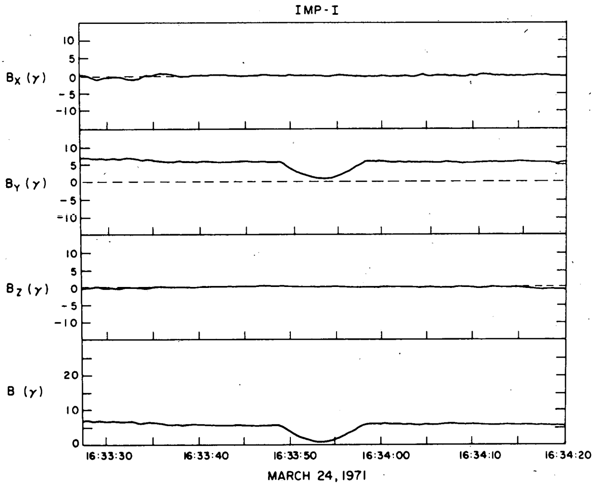
Fig. 5.- A linear magnetic hole. In this case, the hole is certainly not the result of merging. This, and perhaps all magnetic holes might be a diamagnetic effect due to a localized plasma inhomogeneity.
