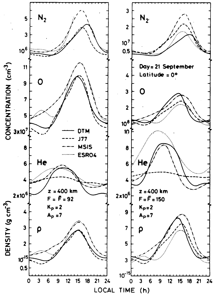
Fig. 5.- Diurnal variation of N_2 , O , He and total density at the equator on 21 September. Altitude = 400 km. Two solar activity levels F = \bar{F} = 92 \times 10^{-22} \text{ W m}^{-2} \text{ Hz}^{-1} and F = \bar{F} = 150 \times 10^{-22} \text{ W m}^{-2} \text{ Hz}^{-1} . Geomagnetic index K_p = 2 or A_p = 7 . For J77 longitude is 0^\circ .
