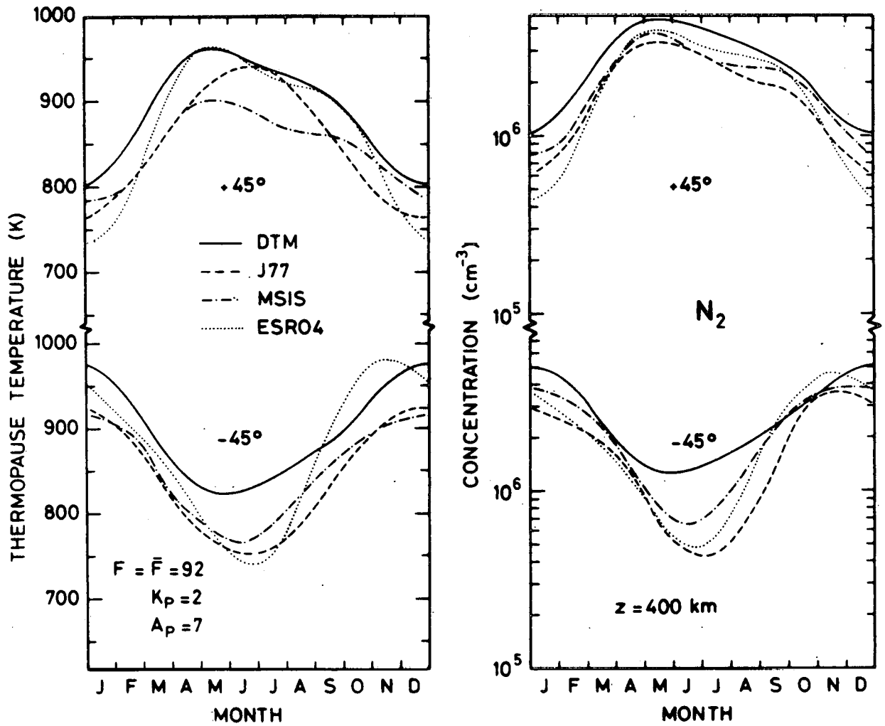
Fig. 7.- Diurnally averaged thermopause temperature and molecular nitrogen concentration at 400 km for \pm 45^\circ latitude. Geomagnetic index K_p = 2 or A_p = 7 . Solar decimetric flux F = \bar{F} = 92 \times 10^{-22} \text{ W m}^{-2} \text{ Hz}^{-1} . Longitude 2.22^\circ\text{E} for J77.
