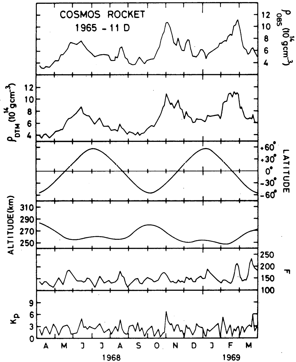
Fig. 1.- Comparison of total densities \rho_{OBS} deduced from drag data of Cosmos Rocket 1965-11D and model densities \rho_{DTM} . Latitude and altitude of satellite perigee are given from April 1968 through March 1969. Daily solar decimetric flux F in 10^{-22} \text{ W m}^{-2} \text{ Hz}^{-1} and geomagnetic index K_p .
