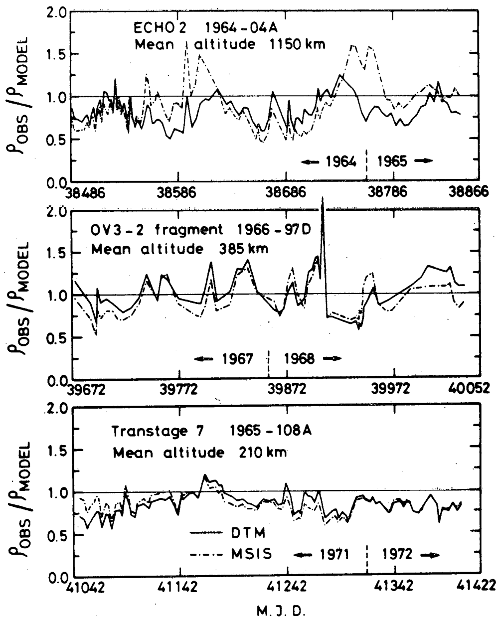
Fig. 12.- Ratio \rho_{\text{OBS}}/\rho_{\text{MODEL}} for three satellites as a function of the modified Julian day (M.J.D.). Model densities are computed respectively with DTM and MSIS.
