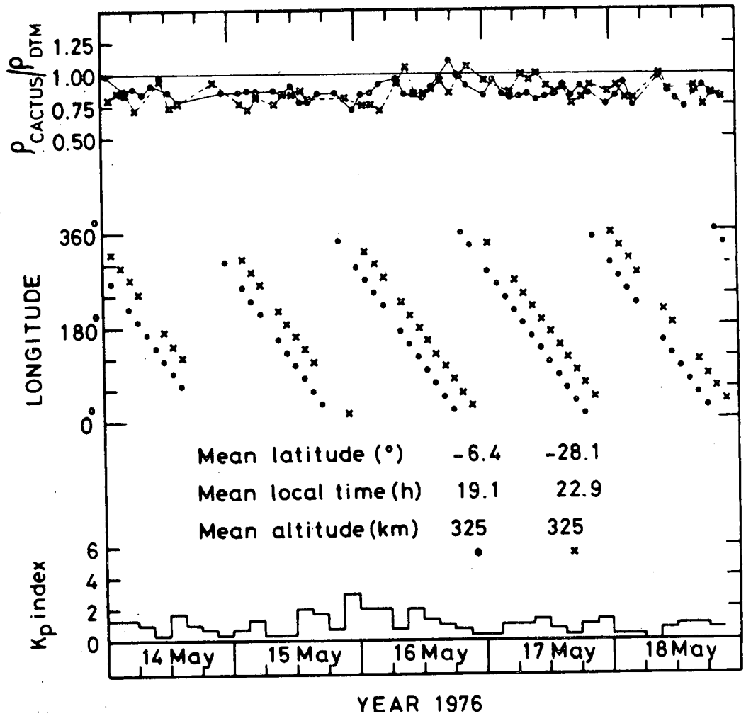
Fig. 14.- Comparison between micro-accelerometer densities \rho_{\text{CACTUS}} and densities obtained from DTM. Longitude of the satellite is indicated as well as K_p indices.
