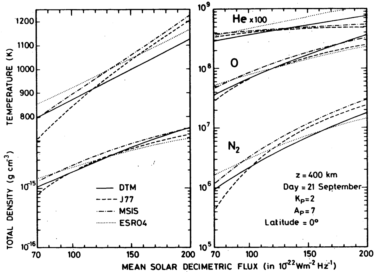
Fig. 2.- Daily averaged thermopause temperature, total density and partial concentrations at the equator as a function of mean solar decimetric flux. Comparison at 400 km between DTM, J77, MSIS and ESRO4 on 21 September for K_p = 2 or A_p = 7 .
