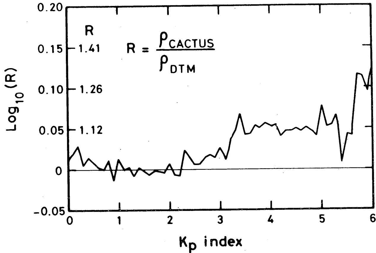
Fig. 15.- Comparison between micro-accelerometer densities \rho_{\text{CACTUS}} and \rho_{\text{DTM}} as a function of geomagnetic index K_p . The CACTUS data are exclusively obtained for low latitudes.
