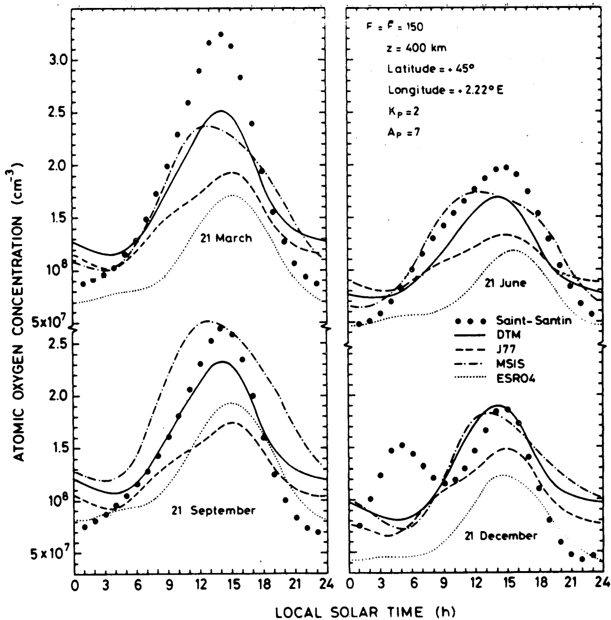
Fig. 6.- Comparison of atomic oxygen incoherent scatter model above Saint-Santin (Alcaydé and Bauer, 1977) with J77, MSIS and DTM for equinox and solstice conditions. Solar activity level F = \bar{F} = 150 \times 10^{-22} \text{ W m}^{-2} \text{ Hz}^{-1} . Geomagnetic index K_p = 2 or A_p = 7 . For J77 longitude is 2.22^\circ \text{E} , i.e. longitude of Saint-Santin.
