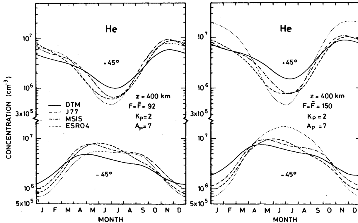
Fig. 10.- Diurnally averaged helium concentration at 400 km for \pm 45^\circ latitude Geophysical conditions identical as in Figs. 7 and 8.
