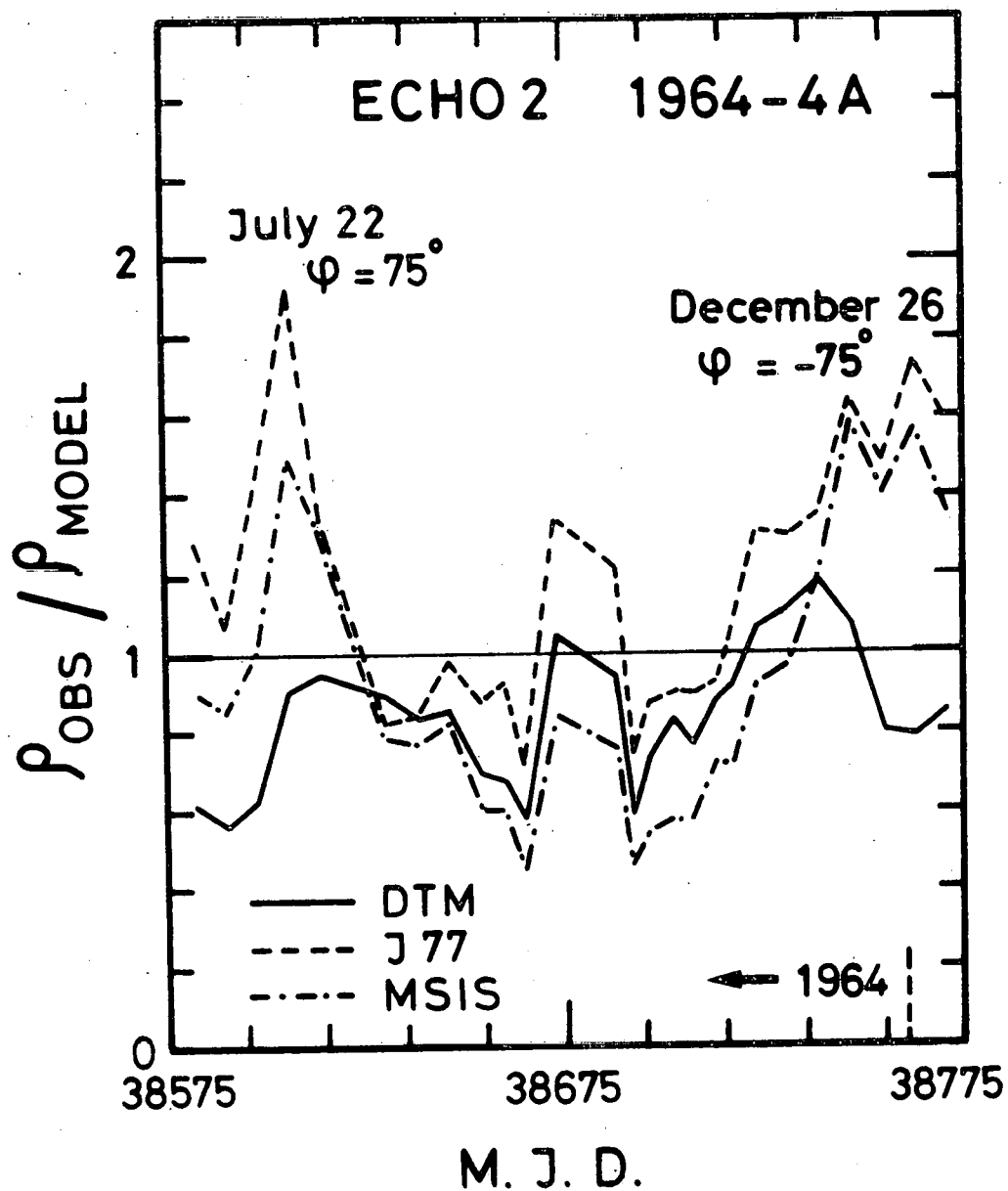
Fig. 13.- Ratio \rho_{OBS}/\rho_{MODEL} for ECHO 2 as a function of the modified Julian day (M.J.D.). Model densities are computed respectively with DTM, MSIS and J77. Perigee latitude is indicated for 22 July 1964 and 26 December 1964.
