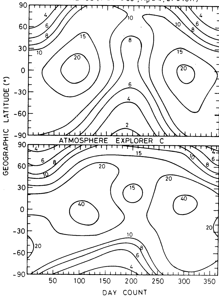
Fig. 6.- Annual variation of atomic nitrogen at 16 hours LT for the same conditions as in Fig. 5.
