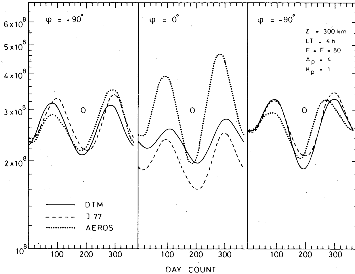
Fig. 2.- Annual variations of atomic oxygen at 300 km computed at 4 hours LT with DTM, J77 and AEROS. Three latitudes are represented, i.e. north and south poles and equator. The daily solar decimetric flux F and the mean flux \bar{F} correspond to the average conditions covered by AEROS. Geomagnetic indices are A_p = 4 or K_p = 1 .
