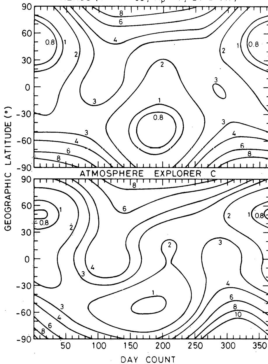
Fig. 5.- Annual variation of atomic nitrogen at 375 km obtained at 4 hours LT for F = \bar{F} = 80 \times 10^{-22} \text{ Wm}^{-2} \text{ Hz}^{-1} and A_p = 4 . Isopleths are in units of 10^5 \text{ cm}^{-3} .
